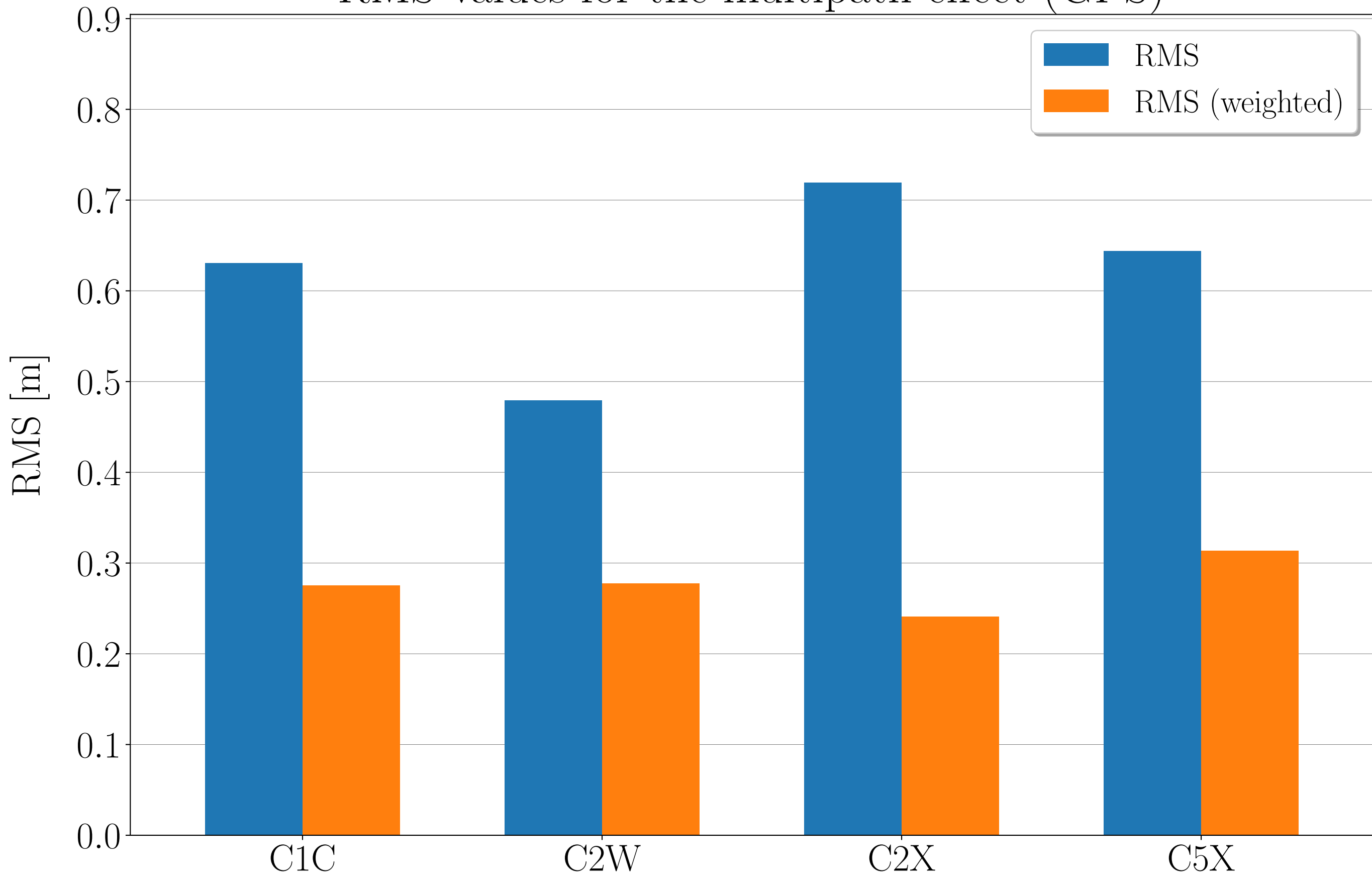
RMS values for the multipath effect (GPS)
