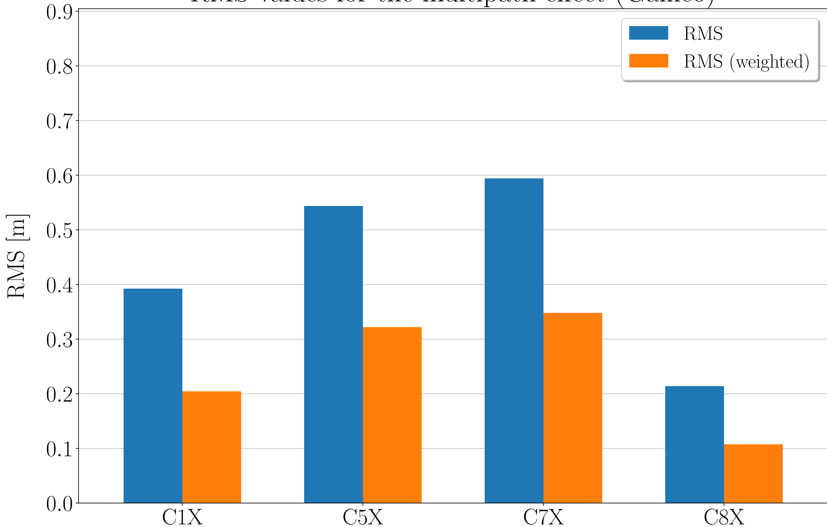
RMS values for the multipath effect (Galileo)
