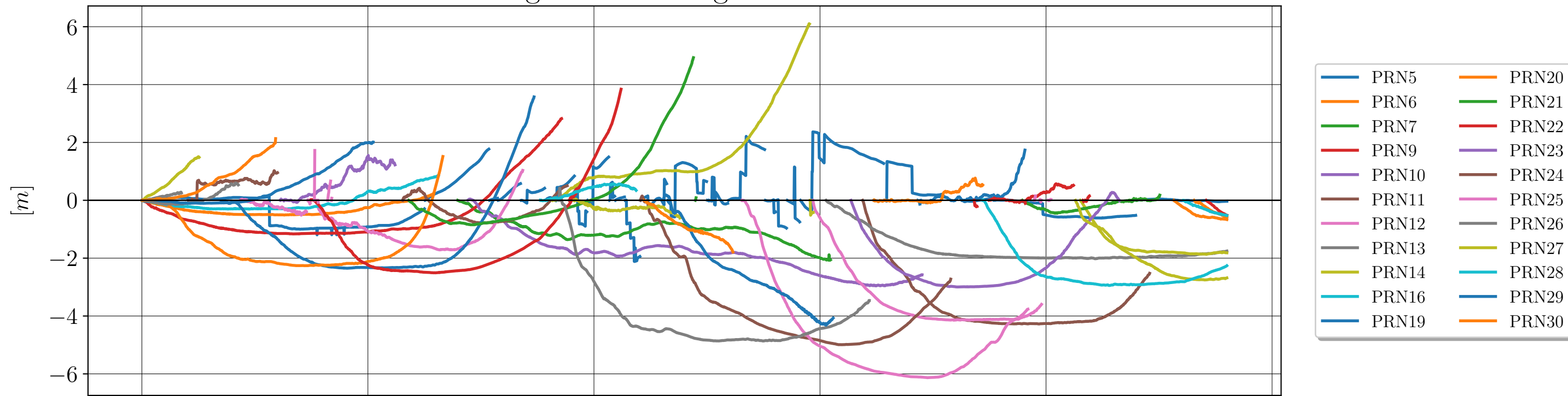
Ionospheric delay vs time for BeiDou
