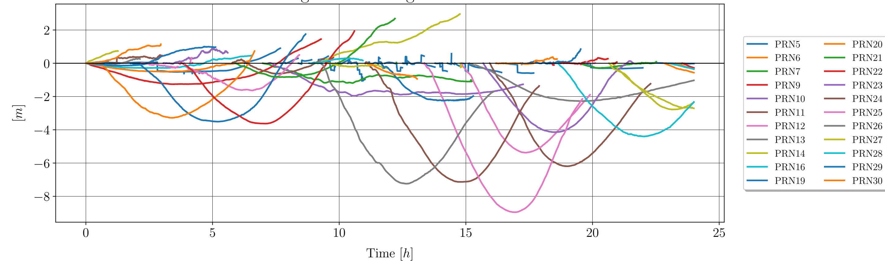
Zenith mapped ionospheric delay for BeiDou
