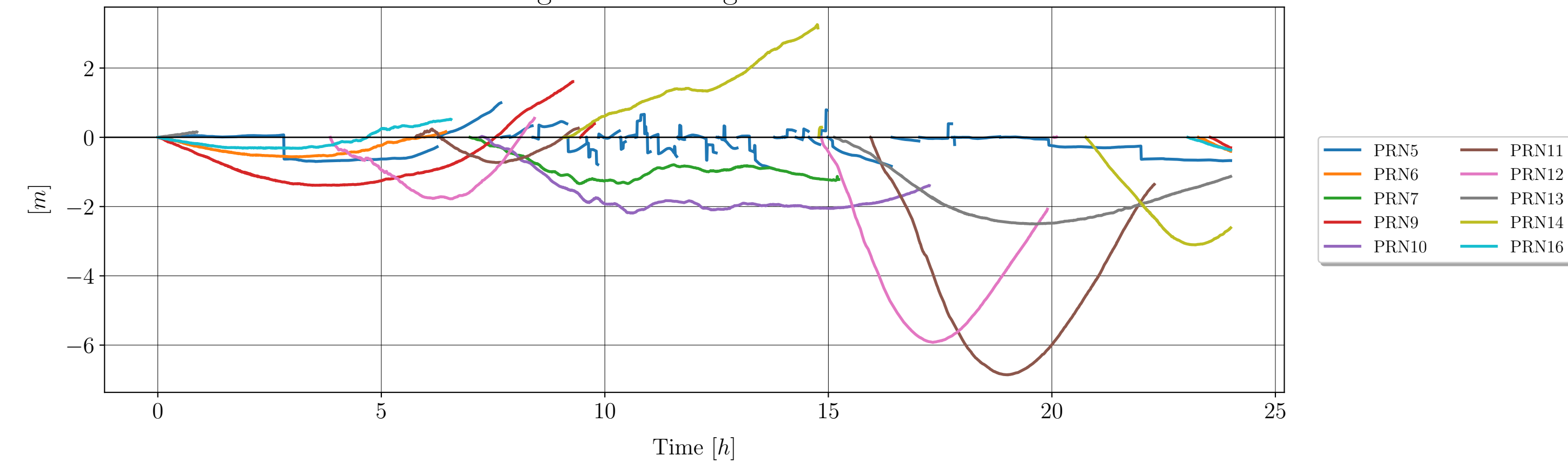
Zenith mapped ionospheric delay for BeiDou
