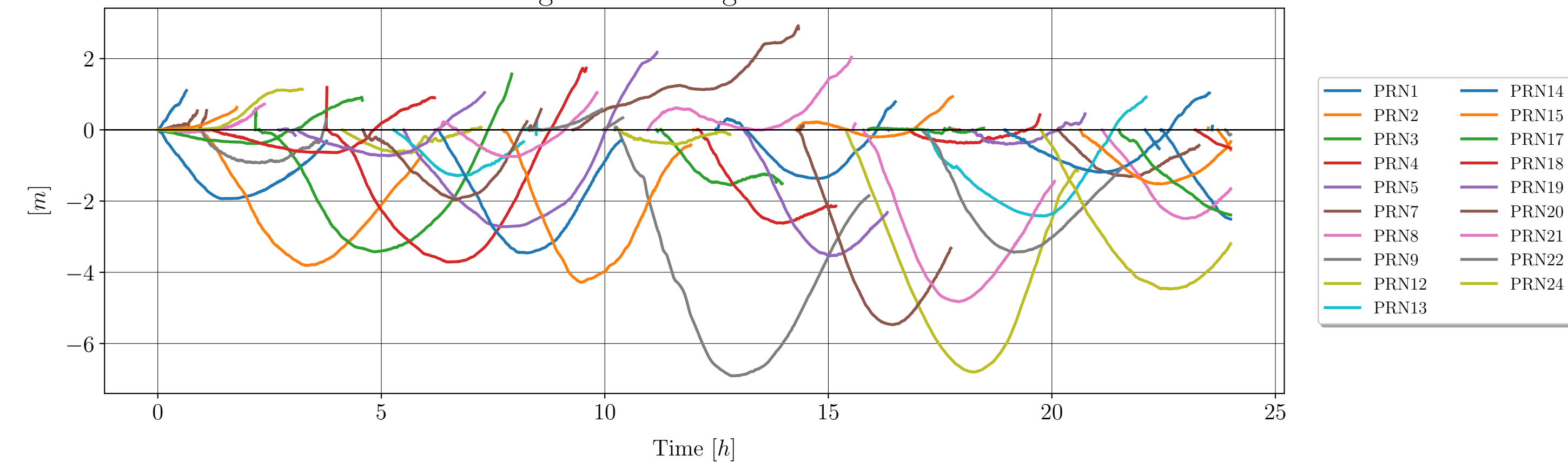
Zenith mapped ionospheric delay for GLONASS
