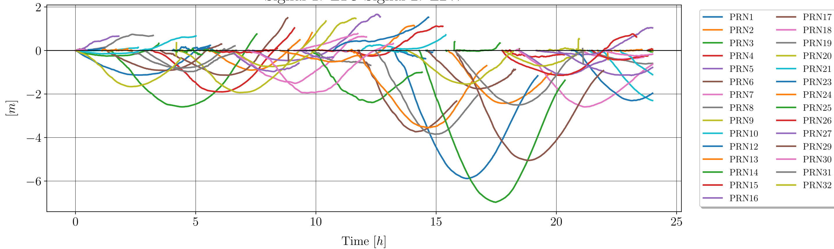
Zenith mapped ionospheric delay for GPS Signal 1: L1C Signal 2: L2W
