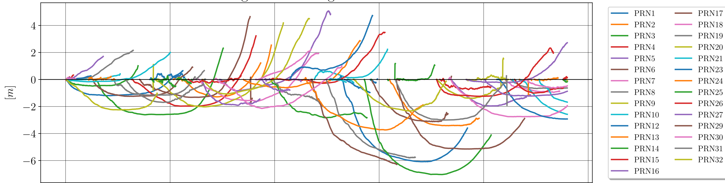
Ionospheric delay vs time for GPS Signal 1: L1C Signal 2: L2W
