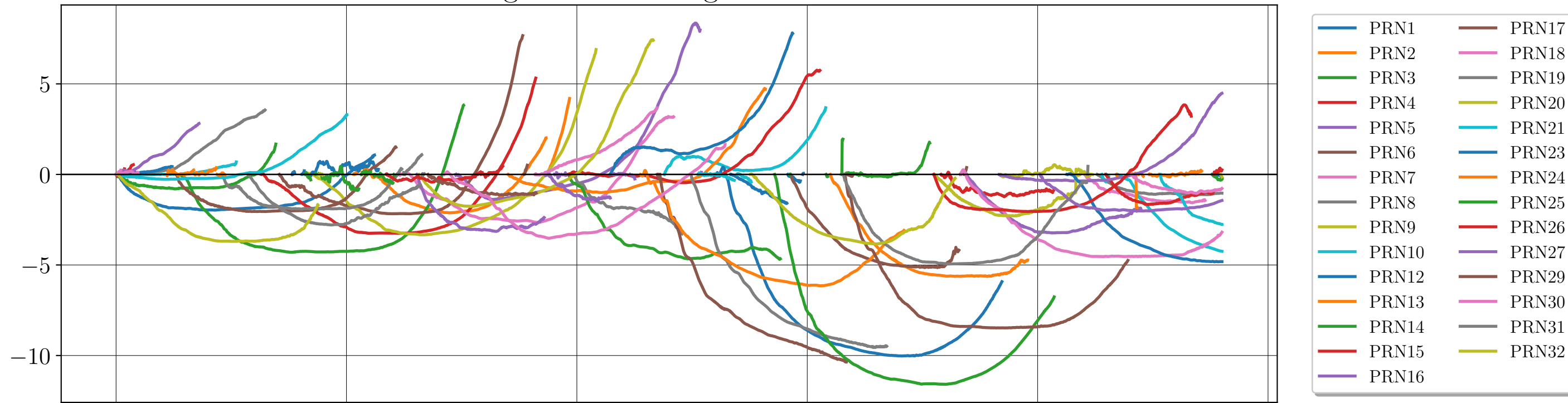
Ionospheric delay vs time for GPS Signal 1: L2W Signal 2: L1C
