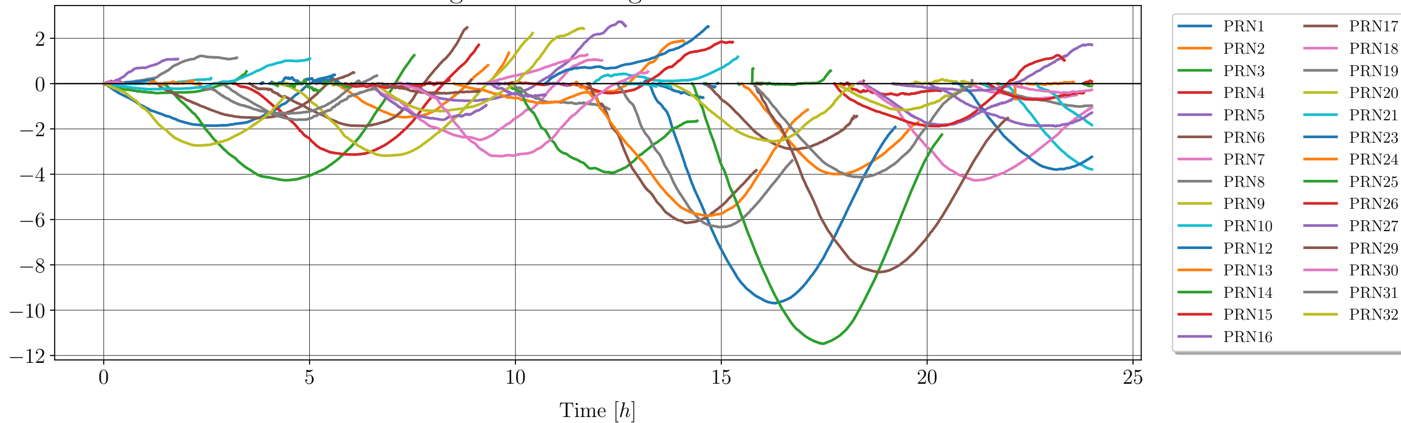
Zenith mapped ionospheric delay for GPS Signal 1: L2W Signal 2: L1C
