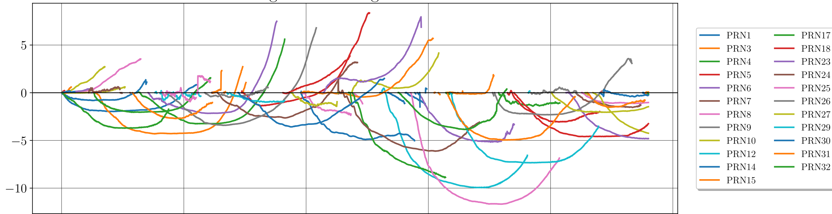
Ionospheric delay vs time for GPS Signal 1: L2X Signal 2: L1C
