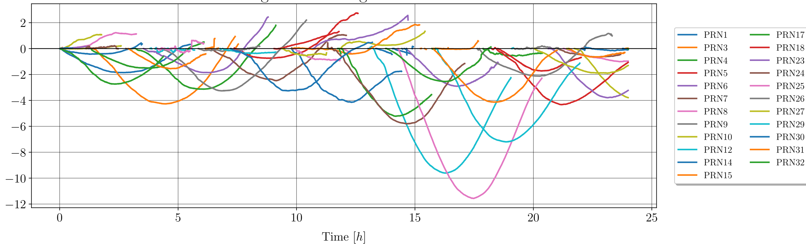
Zenith mapped ionospheric delay for GPS Signal 1: L2X Signal 2: L1C
