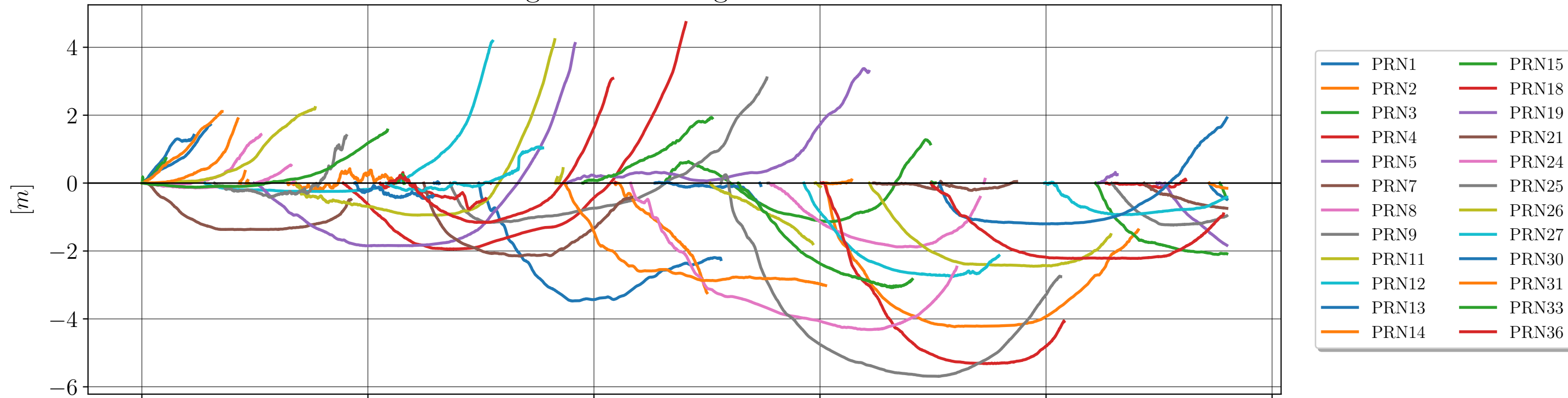
Ionospheric delay vs time for Galileo
