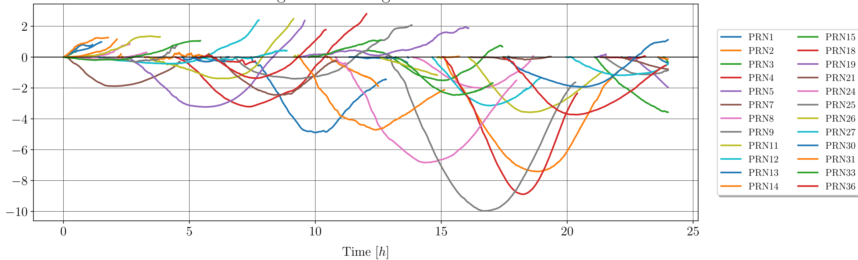
Zenith mapped ionospheric delay for Galileo
