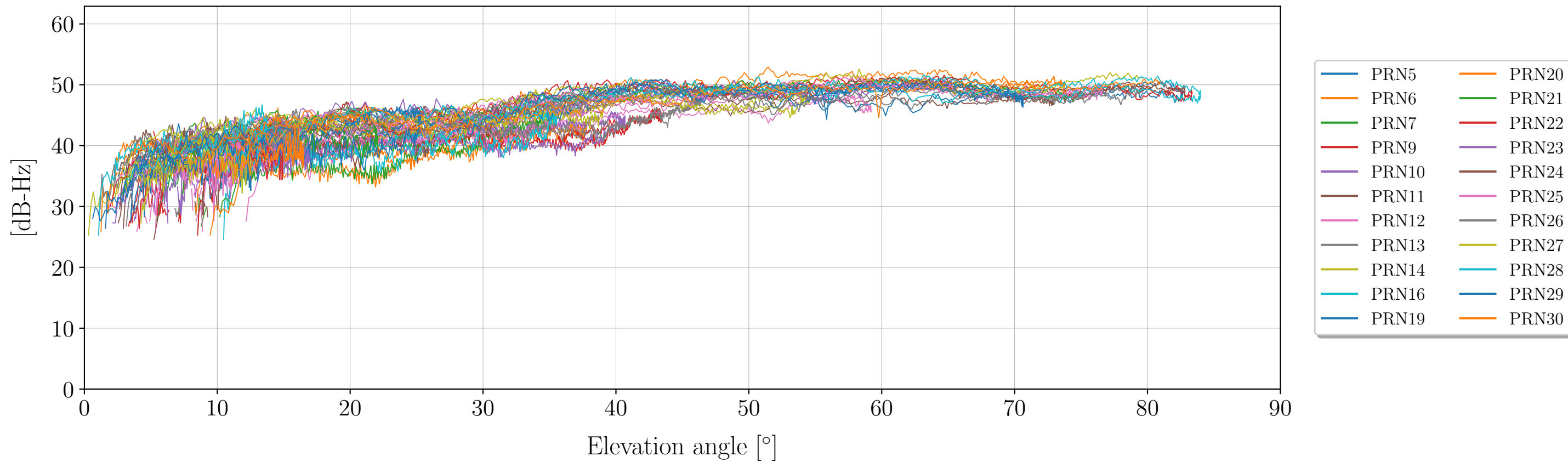
Signal to noise ratio (SNR) as funtion of elevation angle for Signal: S2X (BeiDou)
