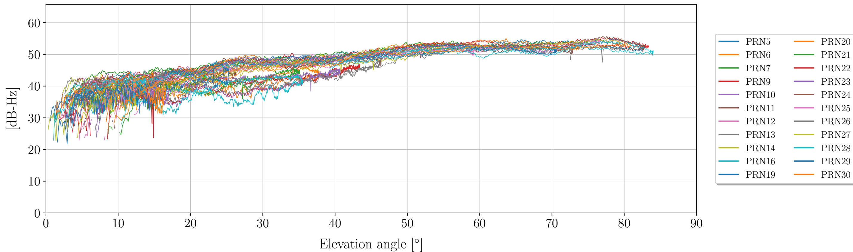
Signal to noise ratio (SNR) as funtion of elevation angle for Signal: S6X (BeiDou)
