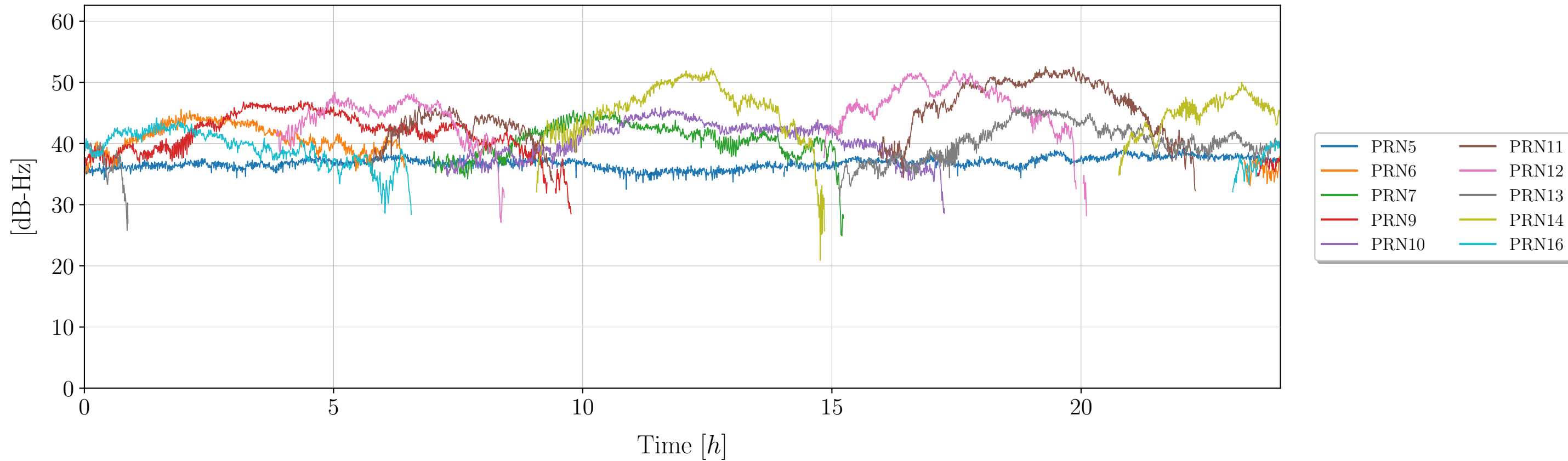
Signal to noise ratio (SNR) as funtion of time for Signal: S7X (BeiDou)
