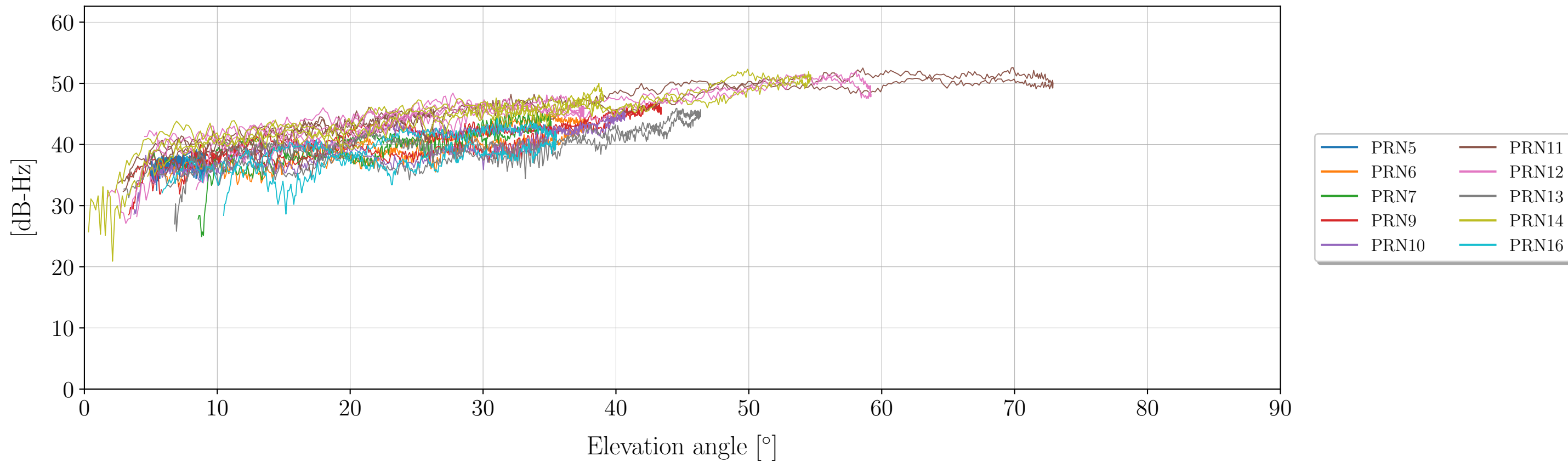
Signal to noise ratio (SNR) as funtion of elevation angle for Signal: S7X (BeiDou)
