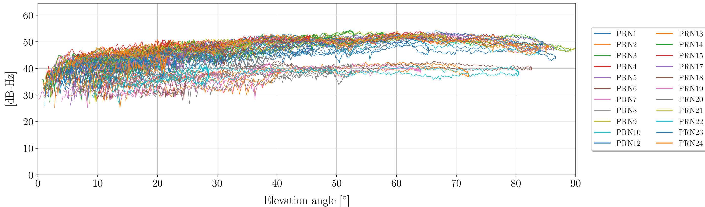
Signal to noise ratio (SNR) as funtion of elevation angle for Signal: S1C (GLONASS)
