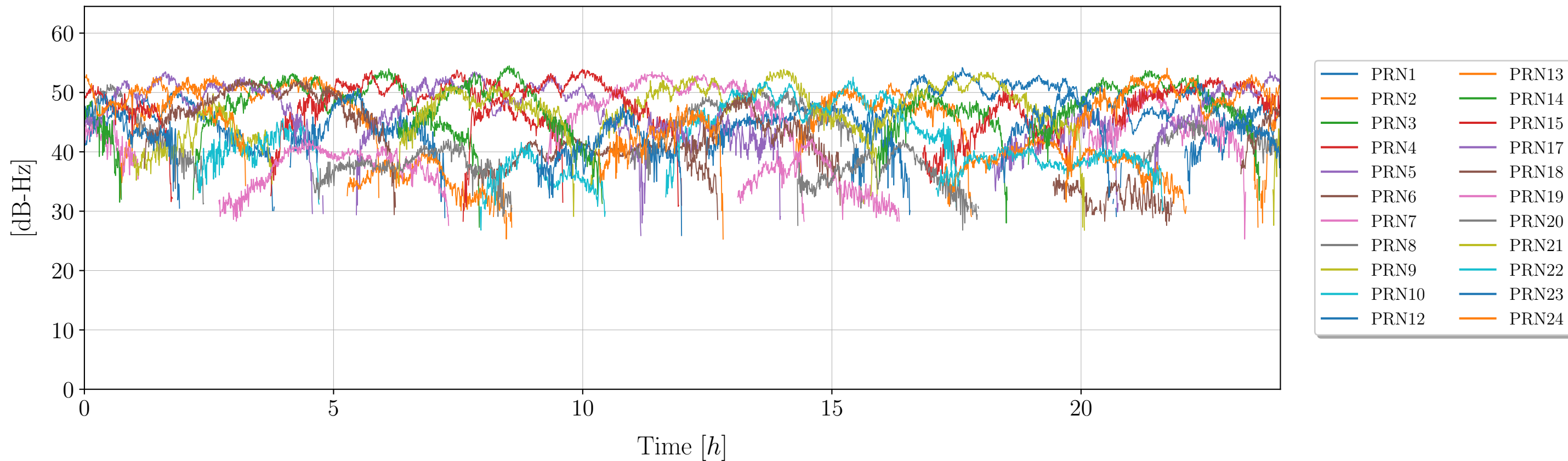
Signal to noise ratio (SNR) as funtion of time for Signal: S1C (GLONASS)
