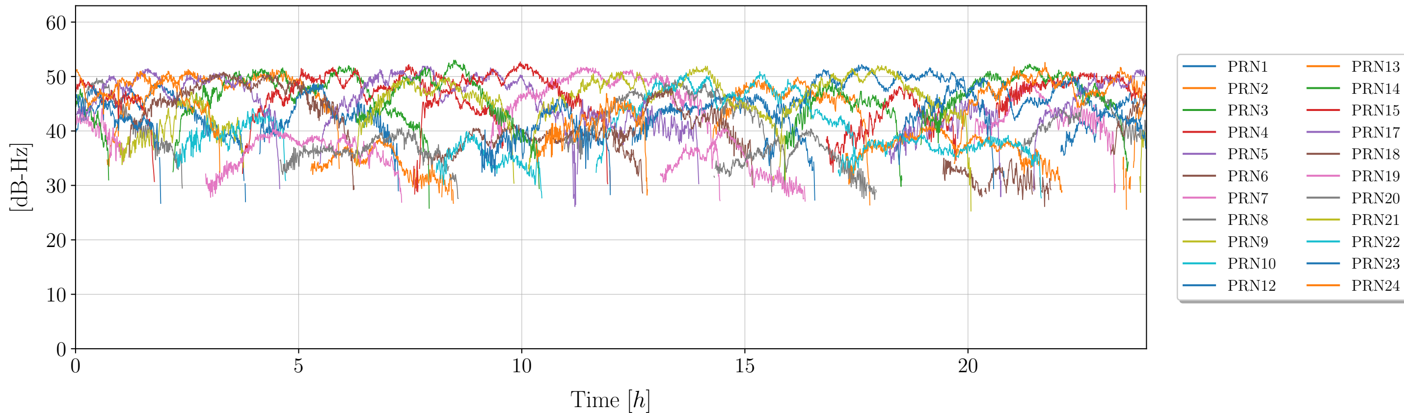
Signal to noise ratio (SNR) as funtion of time for Signal: S1P (GLONASS)
