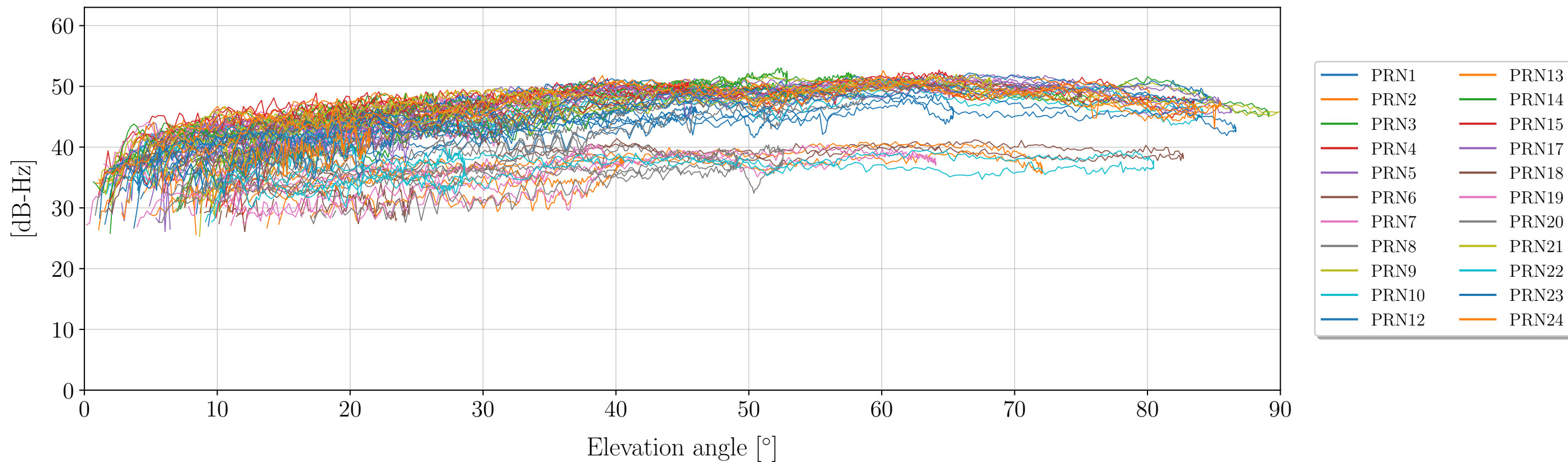
Signal to noise ratio (SNR) as funtion of elevation angle for Signal: S1P (GLONASS)
