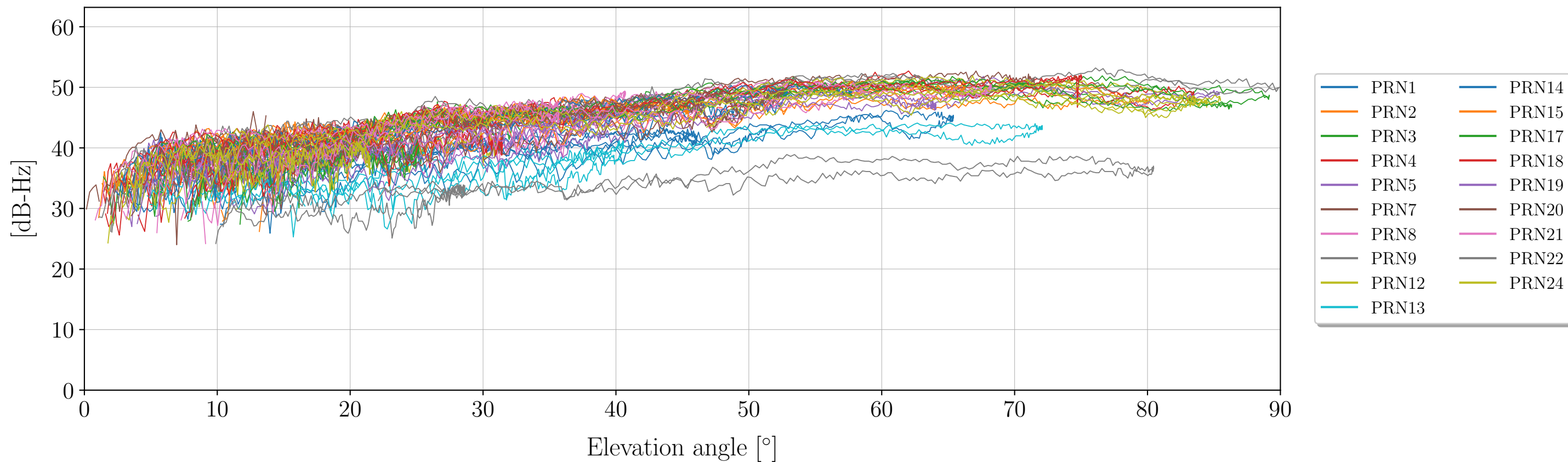
Signal to noise ratio (SNR) as funtion of elevation angle for Signal: S2C (GLONASS)
