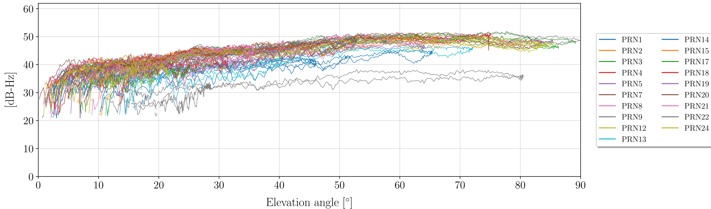
Signal to noise ratio (SNR) as funtion of elevation angle for Signal: S2P (GLONASS)
