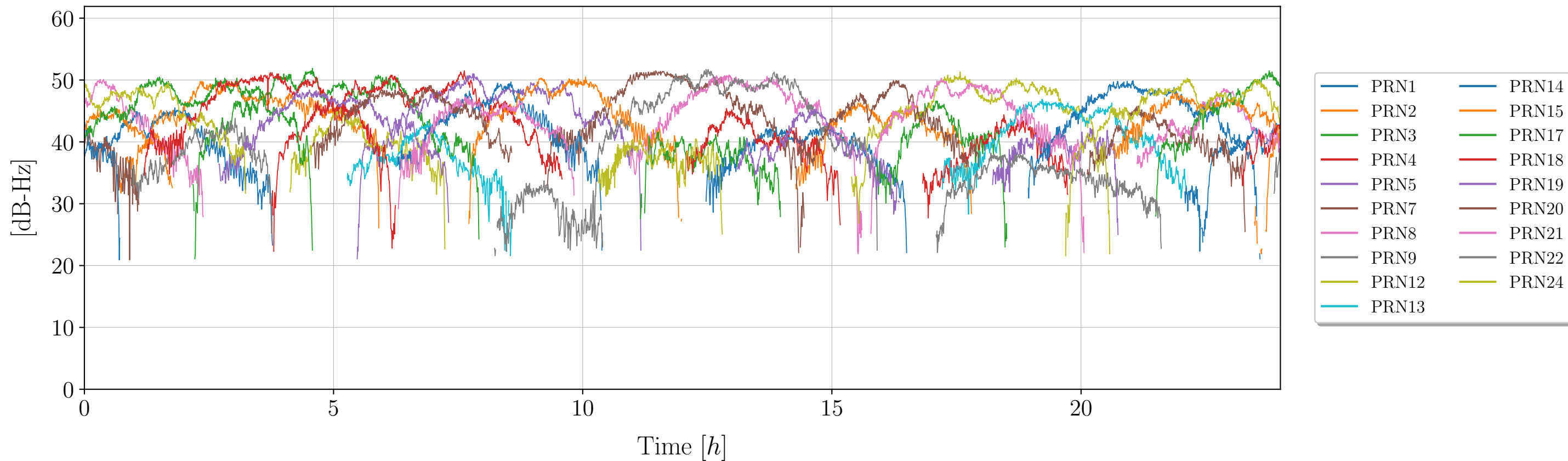
Signal to noise ratio (SNR) as funtion of time for Signal: S2P (GLONASS)
