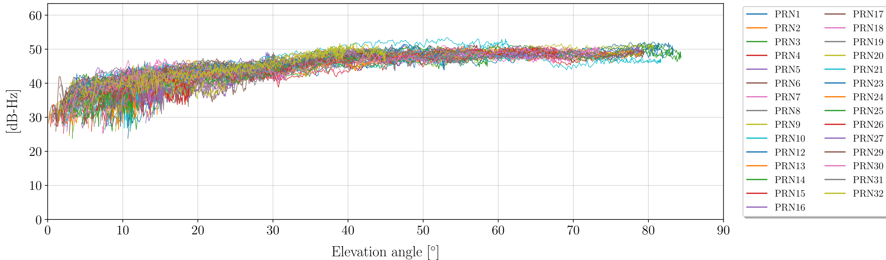
Signal to noise ratio (SNR) as funtion of elevation angle for Signal: S1C (GPS)
