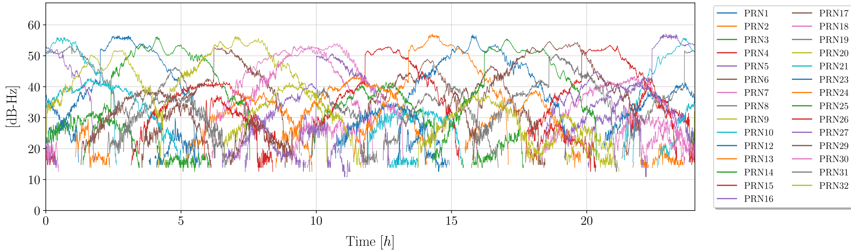
Signal to noise ratio (SNR) as funtion of time for Signal: S2W (GPS)
