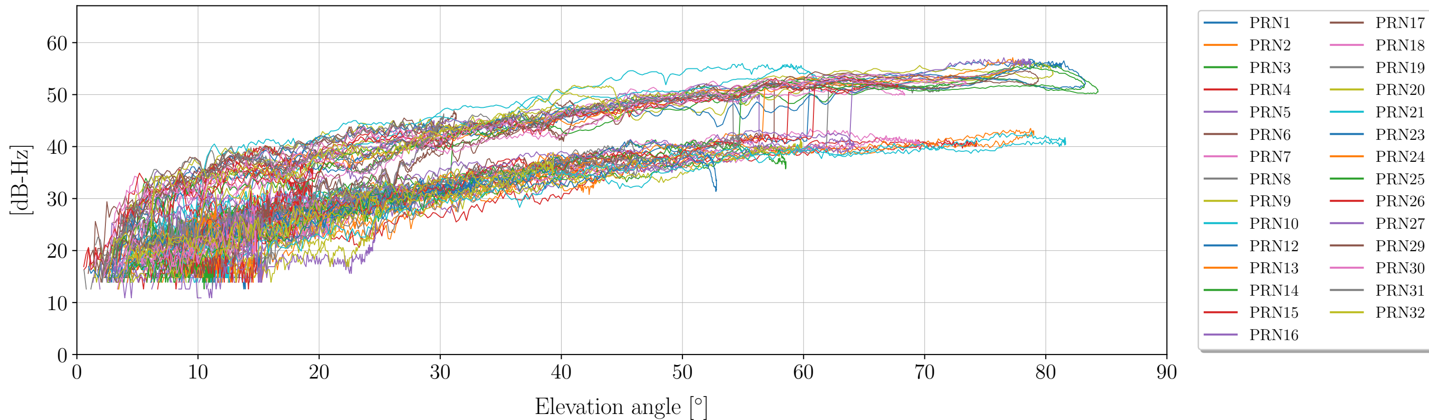
Signal to noise ratio (SNR) as funtion of elevation angle for Signal: S2W (GPS)
