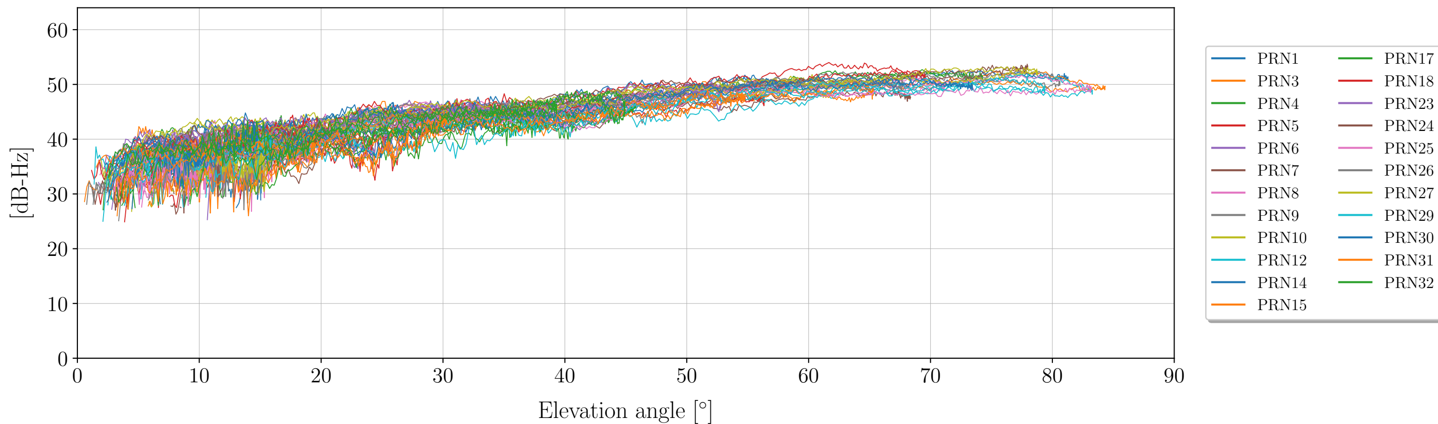
Signal to noise ratio (SNR) as funtion of elevation angle for Signal: S2X (GPS)
