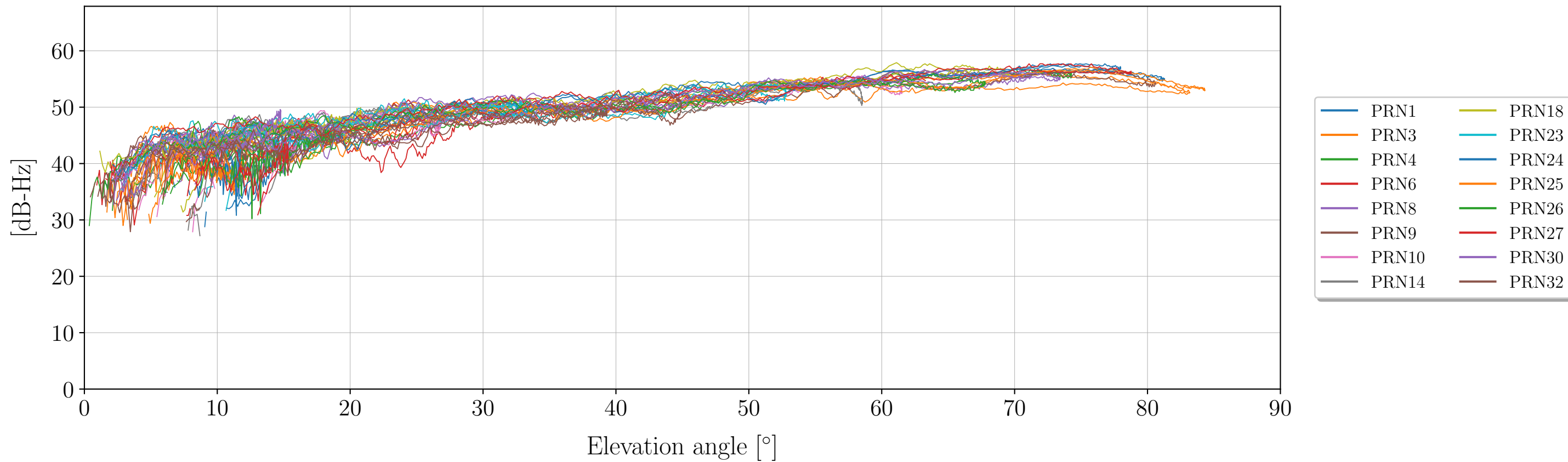
Signal to noise ratio (SNR) as funtion of elevation angle for Signal: S5X (GPS)
