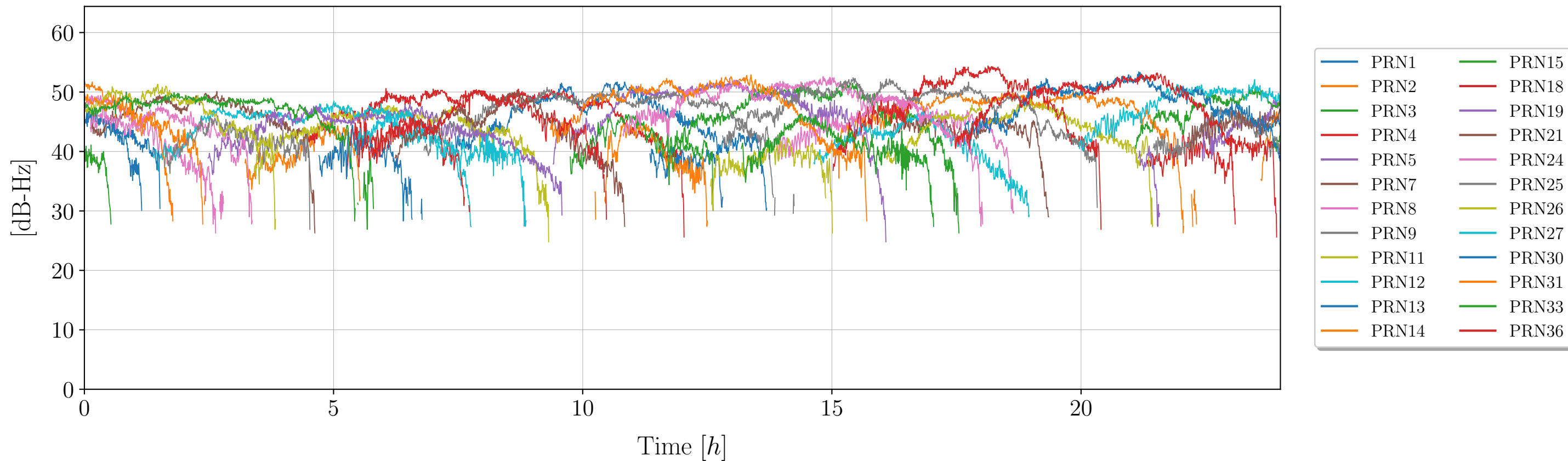
Signal to noise ratio (SNR) as funtion of time for Signal: S1X (Galileo)
