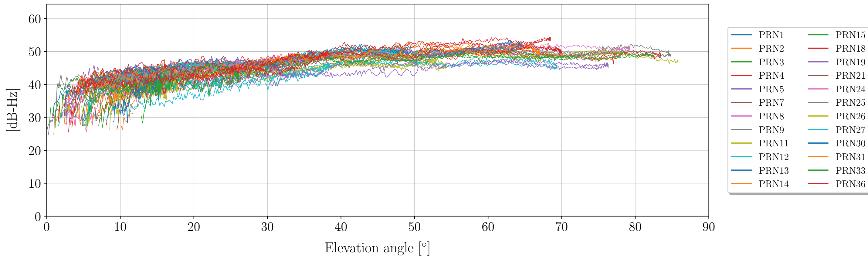
Signal to noise ratio (SNR) as funtion of elevation angle for Signal: S1X (Galileo)
