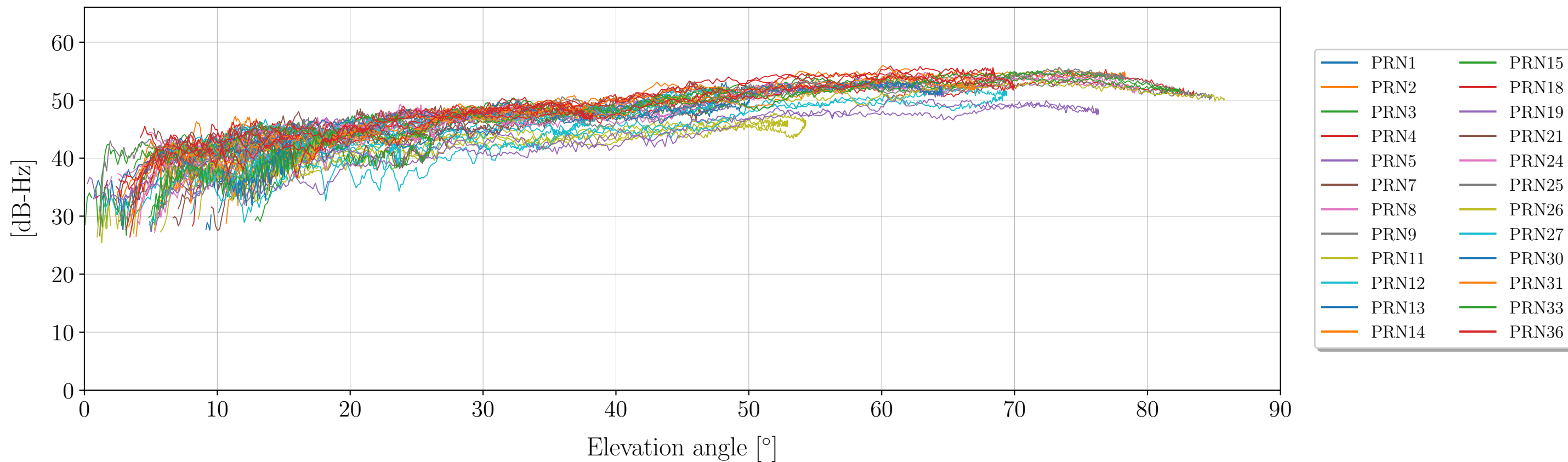
Signal to noise ratio (SNR) as funtion of elevation angle for Signal: S5X (Galileo)
