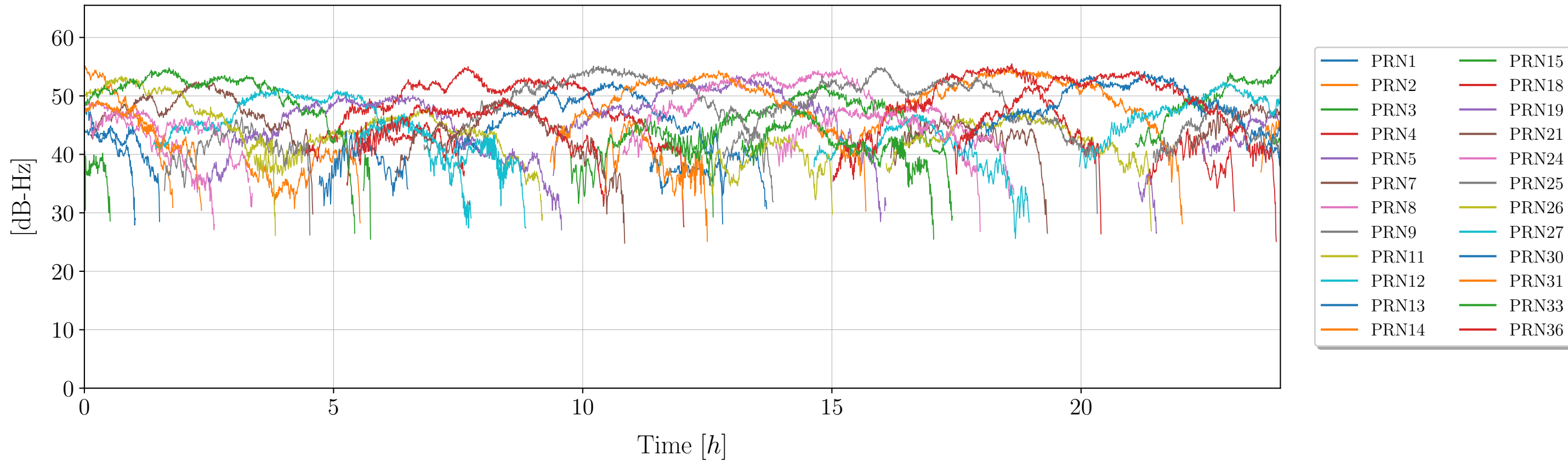
Signal to noise ratio (SNR) as funtion of time for Signal: S7X (Galileo)
