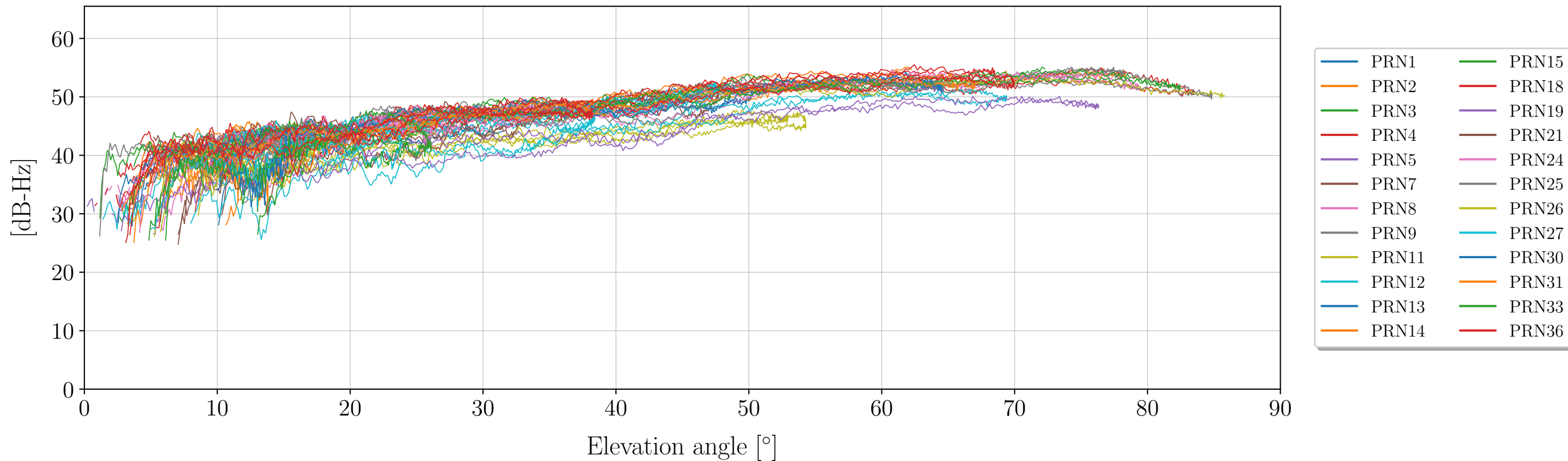
Signal to noise ratio (SNR) as funtion of elevation angle for Signal: S7X (Galileo)
