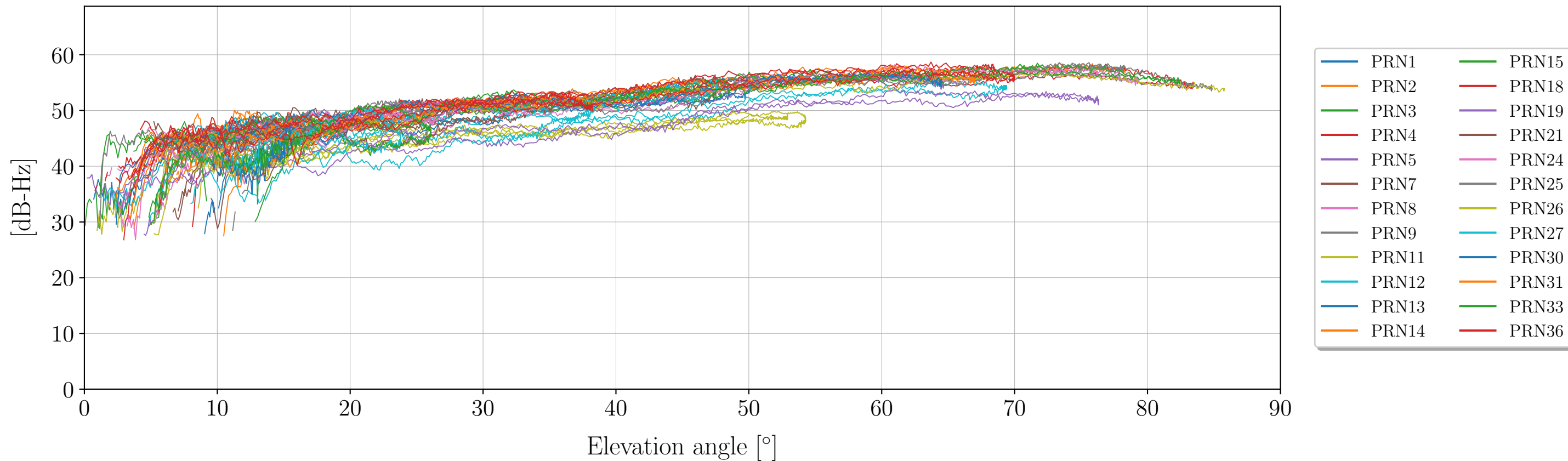
Signal to noise ratio (SNR) as funtion of elevation angle for Signal: S8X (Galileo)
