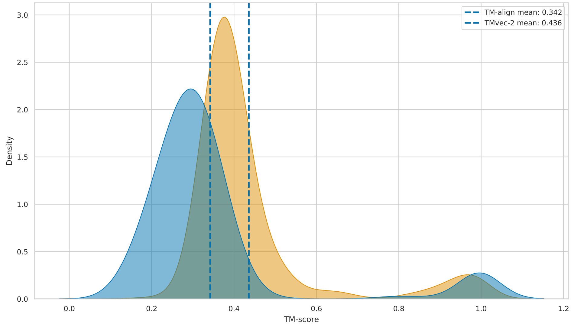
Distribution Comparison: TMvec-2 vs TM-align
