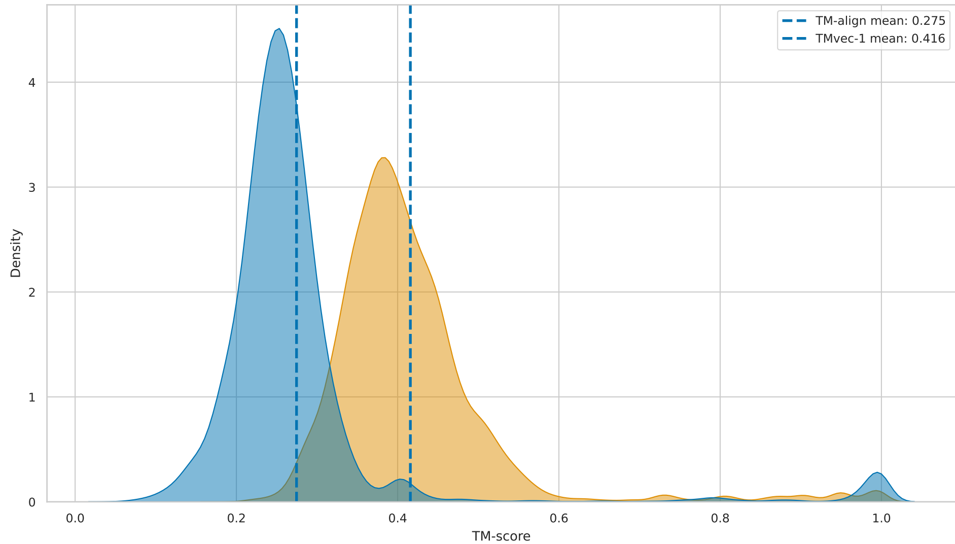
Distribution Comparison: TMvec-1 vs TM-align
