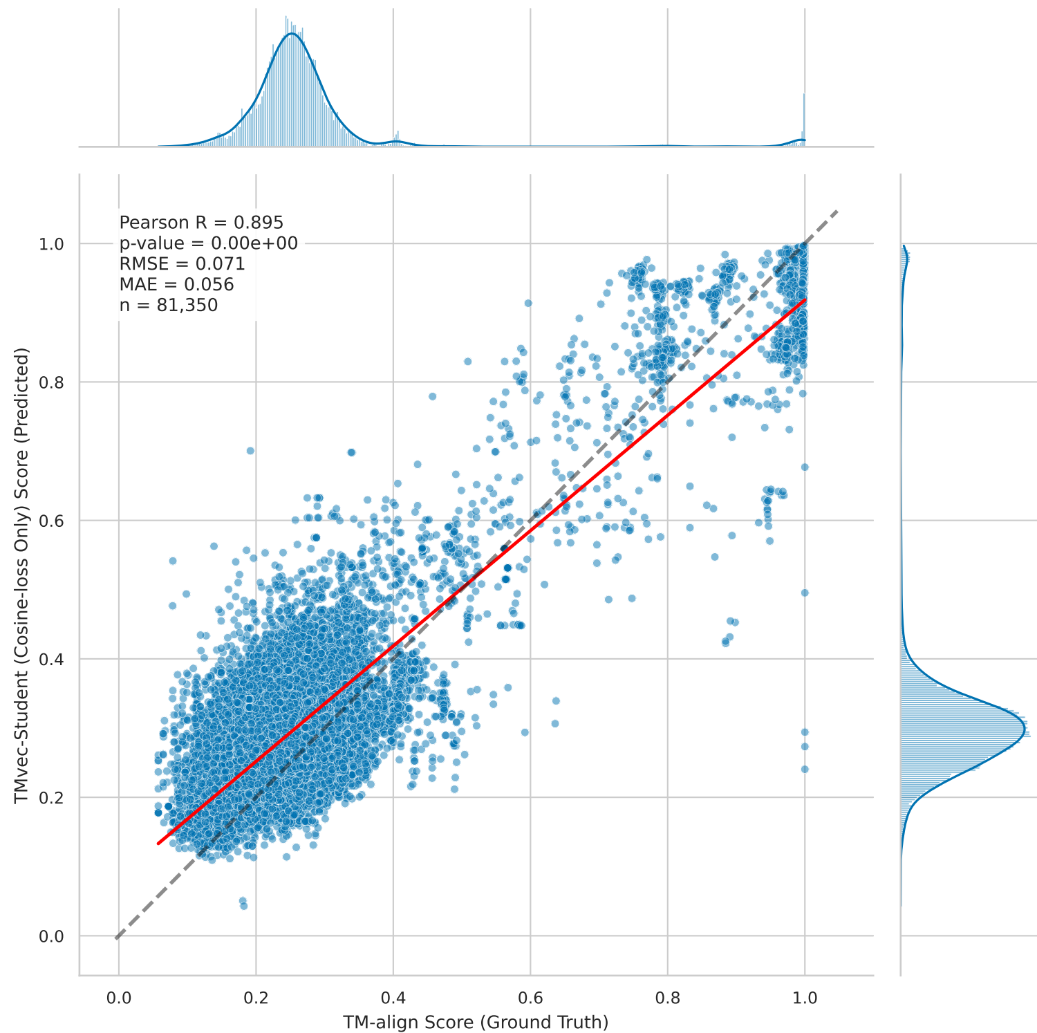
Correlation: TMvec-Student (Cosine-loss Only) vs Ground Truth
