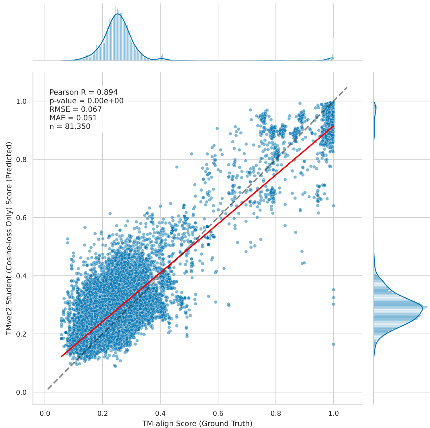
Correlation: TMvec2 Student (Cosine-loss Only) vs Ground Truth
