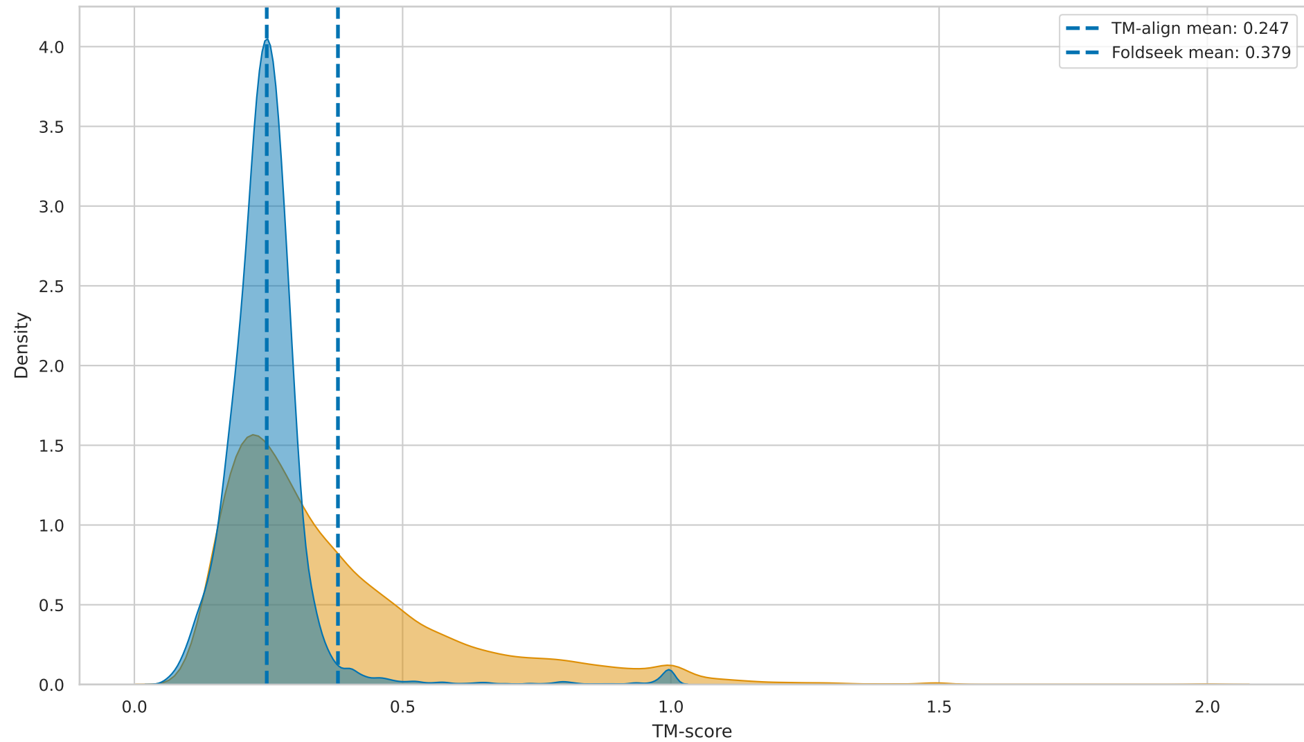
Distribution Comparison: Foldseek vs TM-align
