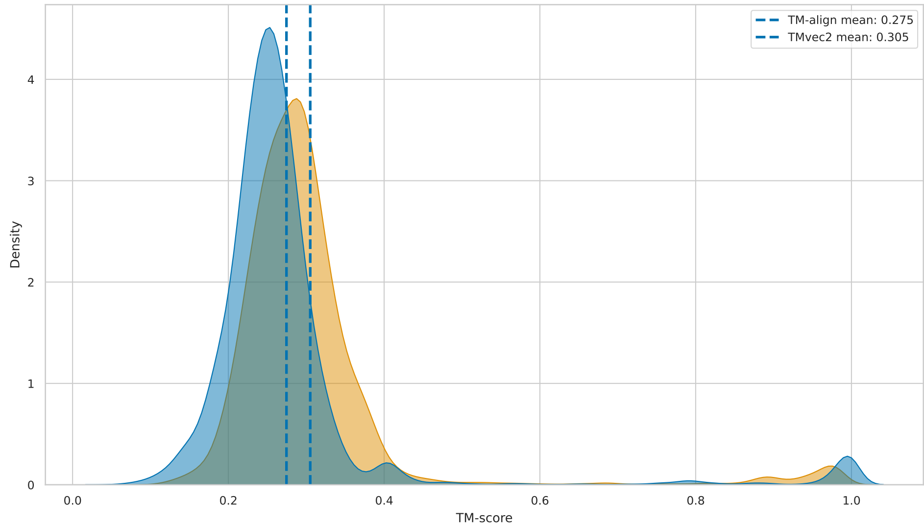
Distribution Comparison: TMvec2 Student (Cosine-loss Only) vs TM-align
