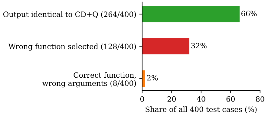
CD+Q+RAG outcome breakdown (7B, 400 test cases)
