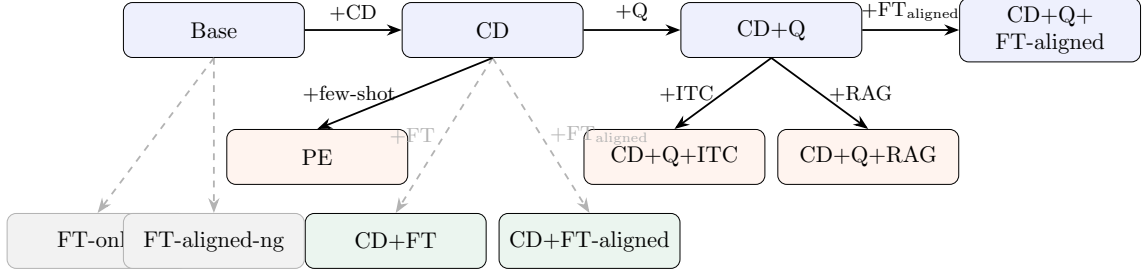
Figure 3.1: Incremental evaluation ladder showing all eleven configurations. The main chain (top row, solid arrows) adds one technique at a time. Orange nodes are inference-time branches: PE branches from CD at full precision; ITC and RAG branch from CD+Q. Green nodes are fine-tuning branches from CD. Gray nodes are unguided standalone configurations (no constrained decoding).
