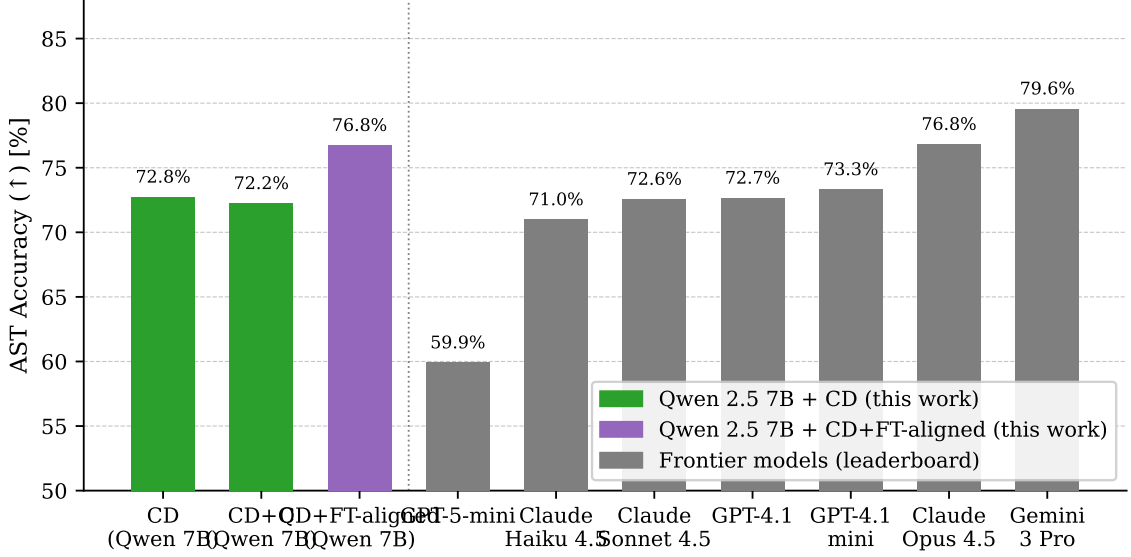
Figure 4.6: BFCL v4 simple.python AST accuracy for Qwen 2.5 7B configurations (this work) vs. frontier models from the official leaderboard (accessed 2026-06-04). CD+FT-aligned reaches 76.75%, within 0.08 pp of Claude Opus 4.5 (76.83%).
