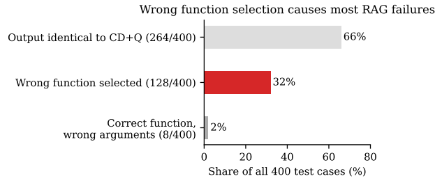
Figure 4.3: Outcome breakdown for CD+Q+RAG on the 7B model over all 400 test cases. The dominant RAG-specific failure mode is wrong function selection (32% of all cases), not retrieval miss or argument extraction error; 66% of outputs are identical to CD+Q.
