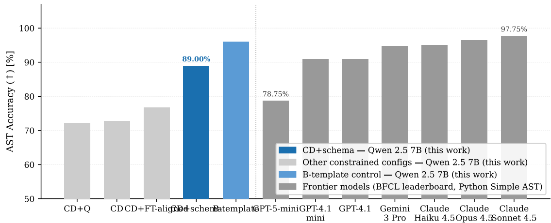
Figure 4.6: BFCL v4 simple_python AST accuracy for Qwen 2.5 7B configurations (this work) vs. frontier models from the official leaderboard (Python Simple AST category). The native-template control (B-template, 96.00%) lies within the flagship frontier band; CD+schema (89.00%) enters the frontier range above GPT-5-mini.
