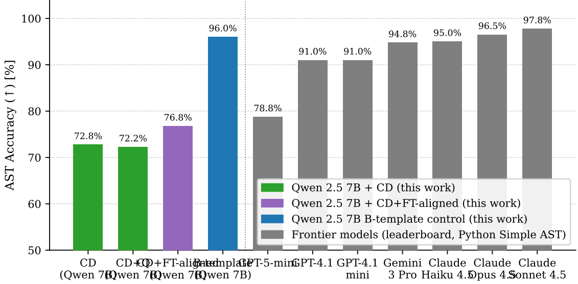
Figure 4.6: BFCL v4 simple_python AST accuracy for Qwen 2.5 7B configurations (this work) vs. frontier models from the official leaderboard (Python Simple AST category). The native-template control (B-template, 96.00%) lies within the flagship frontier band; the best constrained configuration (CD+FT-aligned, 76.75%) is within single-run uncertainty of GPT-5-mini (78.75%).
