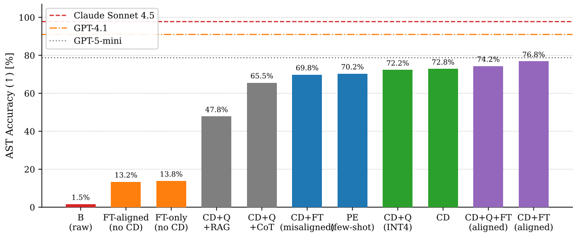
Figure 4.5: BFCL v4 simple_python AST accuracy for all eleven configurations. Dashed reference lines show Claude Sonnet 4.5 (97.75%), GPT-4.1 (91.00%), and GPT-5-mini (78.75%) on the same category (Python Simple AST). CD+FT-aligned and CD+Q+FT-aligned are the only configurations to exceed the no-training ceiling established by Config CD.
