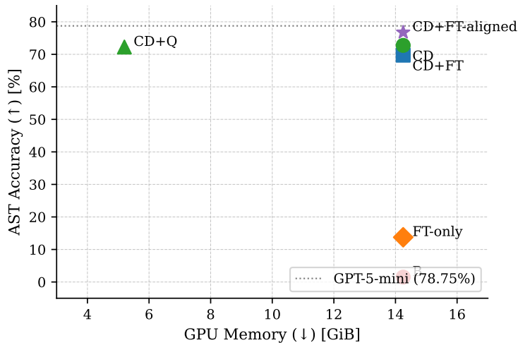
Figure 4.1: GPU memory footprint vs. BFCL simple_python AST accuracy for selected configurations. CD+Q achieves equivalent accuracy to CD at 63.5% lower memory. The reference line marks the weakest frontier entry on this category (GPT-5-mini, 78.75%).
