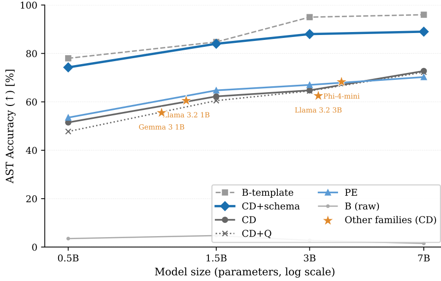
Figure 4.7: BFCL v4 simple_python AST accuracy versus Qwen 2.5 model size (log scale) for the main configurations (Table 4.13). Stars mark Config CD on four other instruct families at their approximate parameter count (Table 4.14); they fall within the Qwen 2.5 CD band by capacity, not by lab. CD+Q overlaps CD throughout, showing the negligible INT4 quantization penalty above 1.5B.
