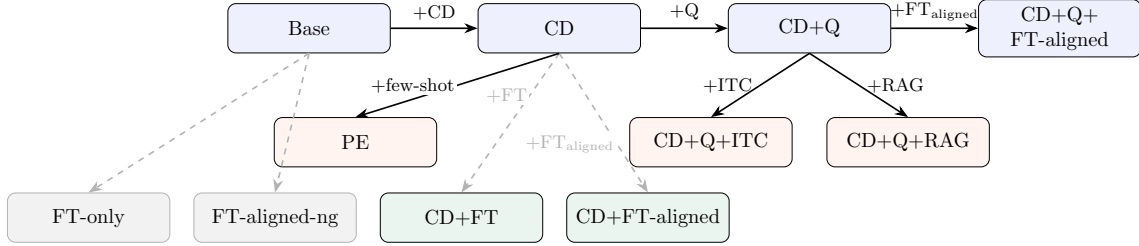
Figure 3.1: Incremental evaluation ladder showing all eleven configurations. The main chain (top row, solid arrows) adds one technique at a time. Orange nodes are inference-time branches: PE branches from CD at full precision; ITC and RAG branch from CD+Q. Green nodes are fine-tuning branches from CD. Gray nodes are unguided standalone configurations (no constrained decoding). The off-ladder CD+schema variant (Section 4.2.3) is evaluated separately and is not shown.
