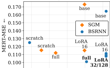
GenSVS/EARS-WHAM
