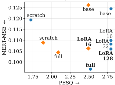
MSRBench/EARS-WHAM
