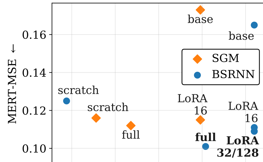
GenSVS/EARS-WHAM
