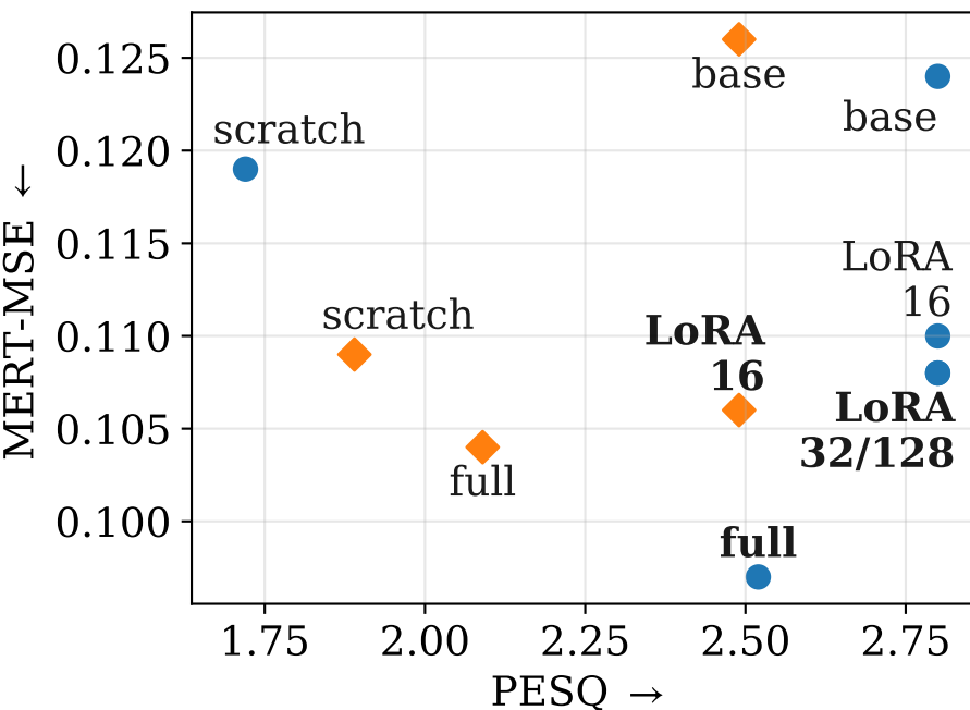
MSRBench/EARS-WHAM
