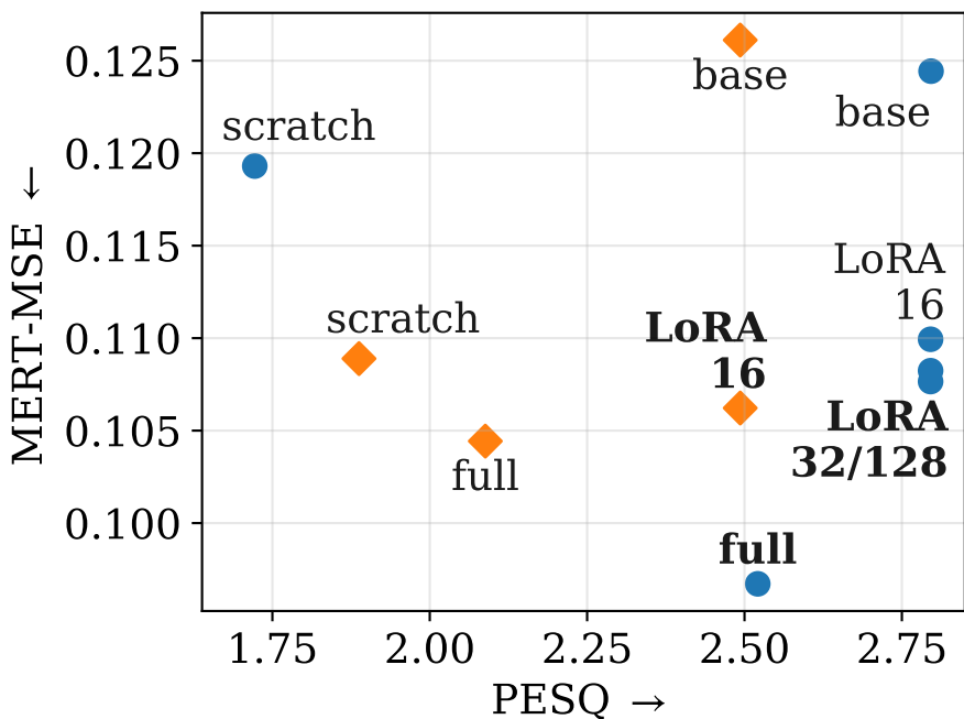
MSRBench/EARS-WHAM
