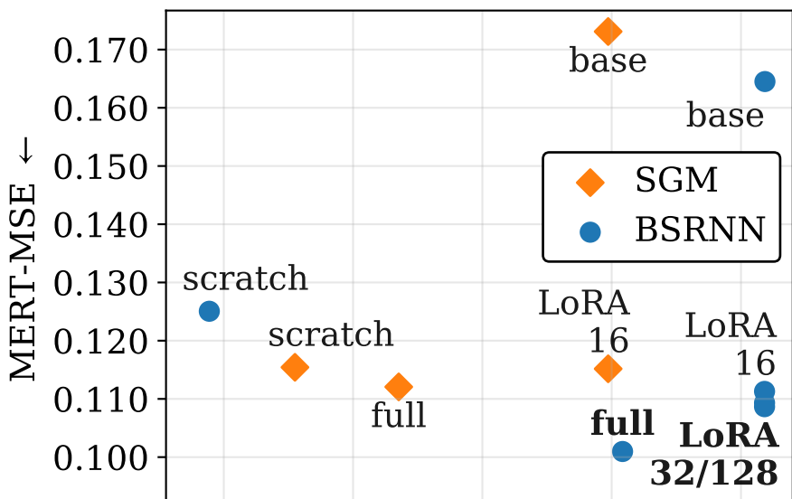
GenSVS/EARS-WHAM
