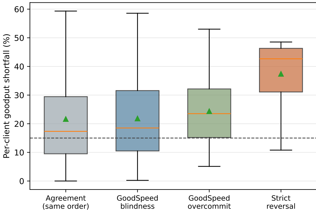
Utility gap by mechanism (box = IQR, triangle = mean)
