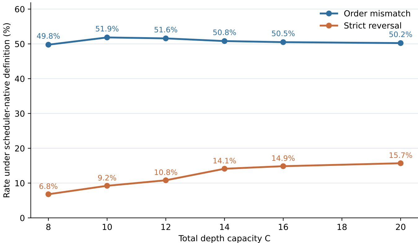
Native-order reversal remains under aggressive capacity
