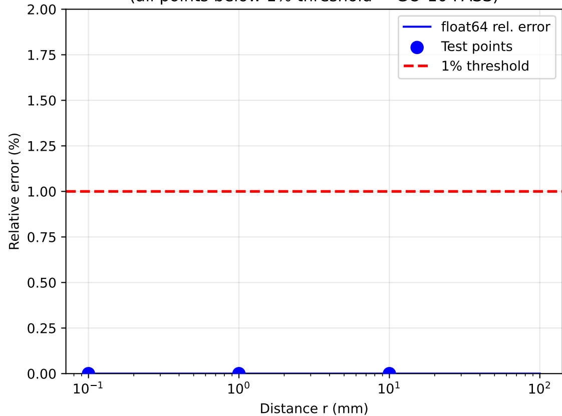
LFP Kernel Accuracy (all points below 1% threshold = GO-10 PASS)
