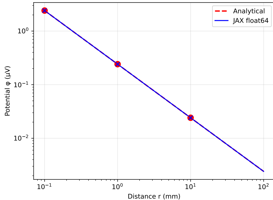
LFP Kernel: \phi vs r ( I = 1 nA, \sigma = 0.33 S/m)
