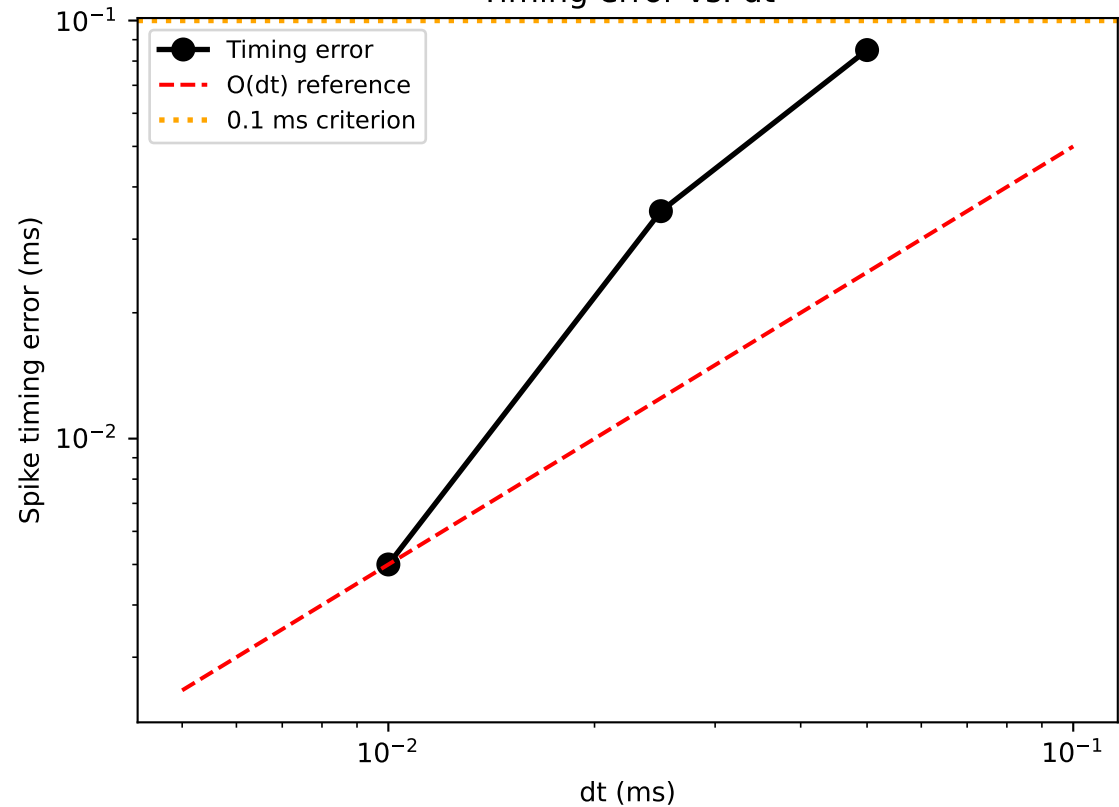
Timing error vs. dt
