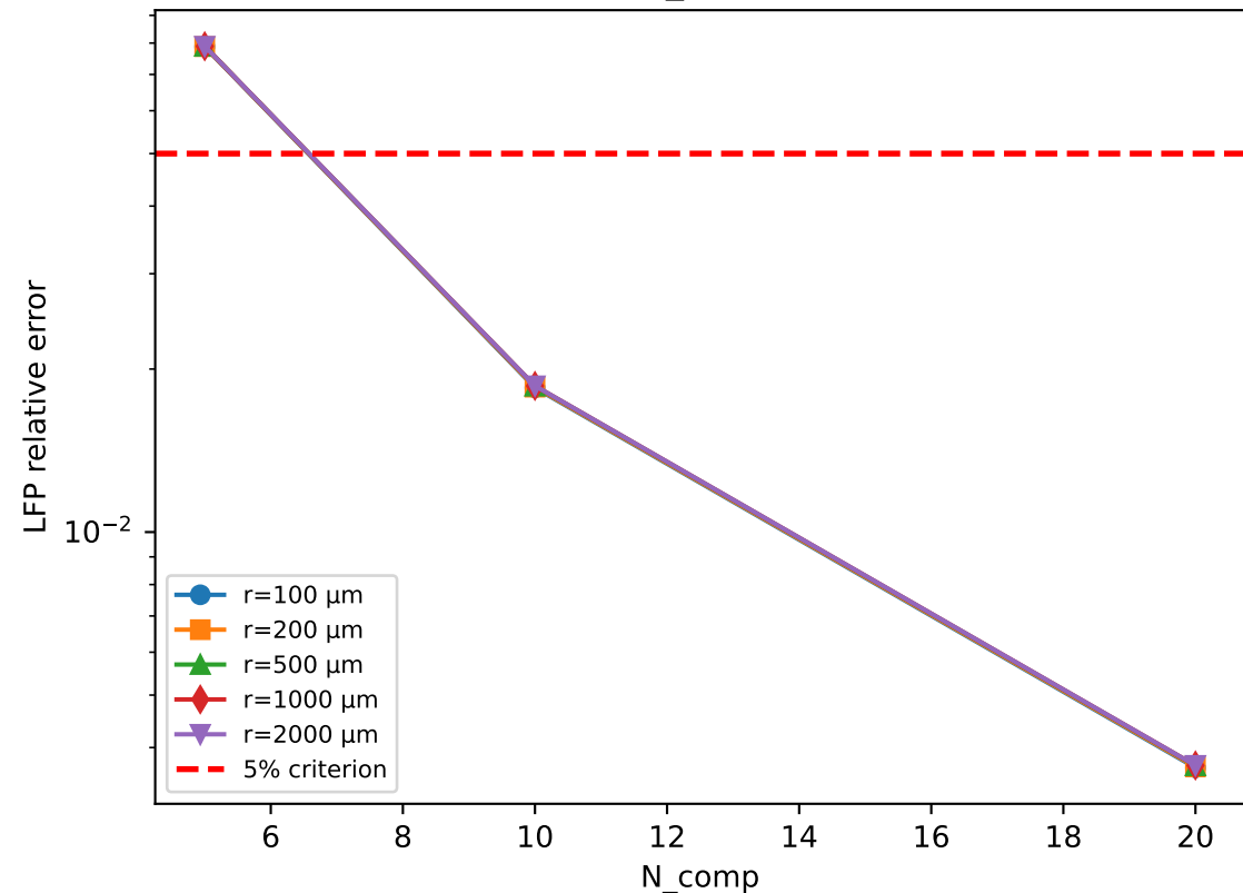
LFP error vs. N_{\text{comp}} (ref: N=40 )
