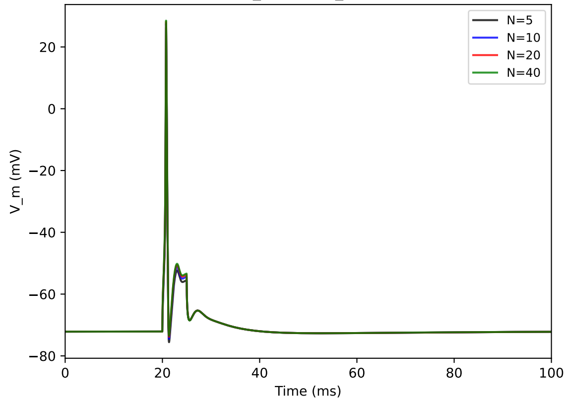
Somatic V_m for 4 N_{\text{comp}} values
