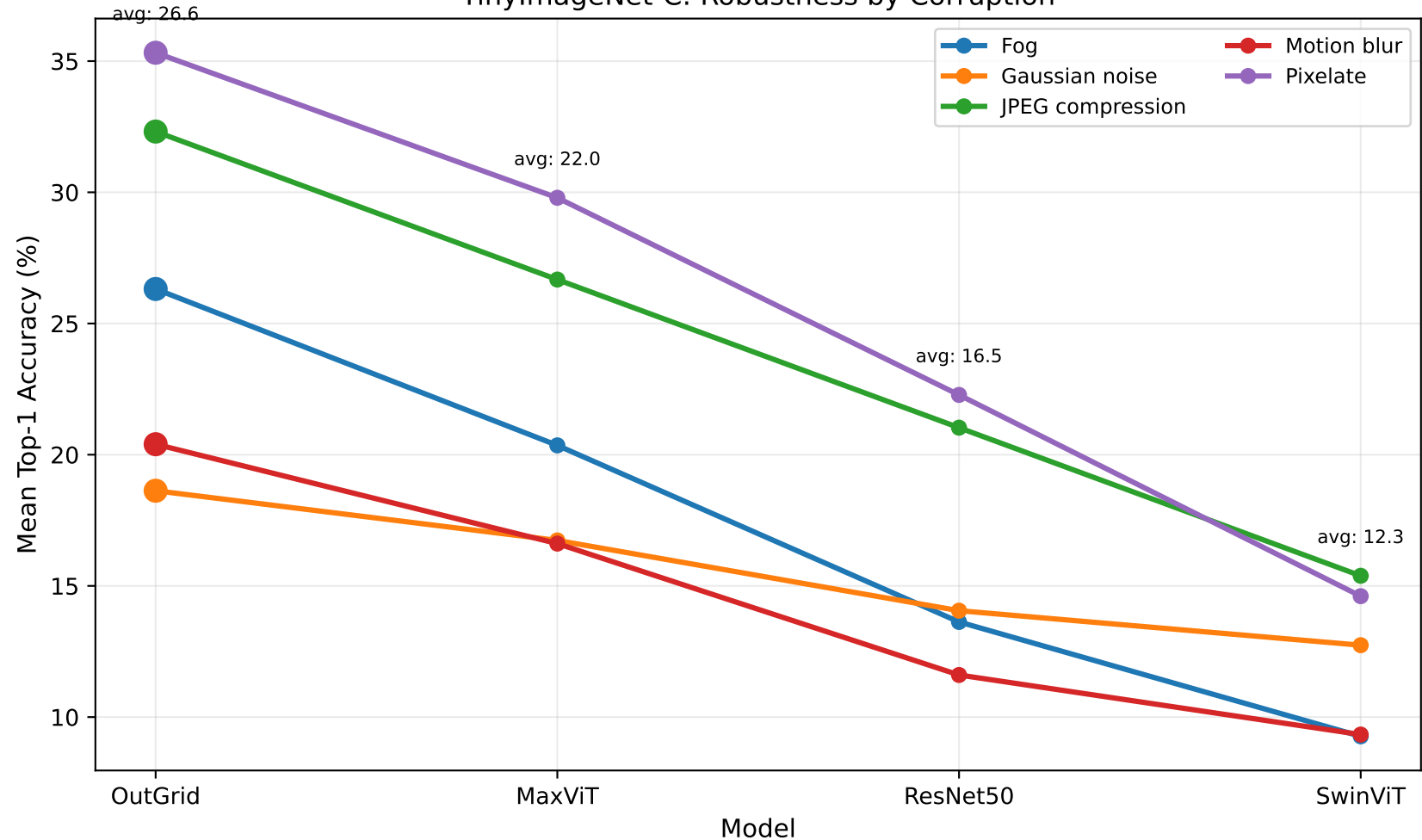
TinyImageNet-C: Robustness by Corruption
