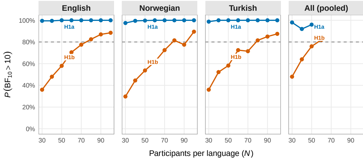
Bayesian Power Curves for the Two Focal Hypotheses, by Language
