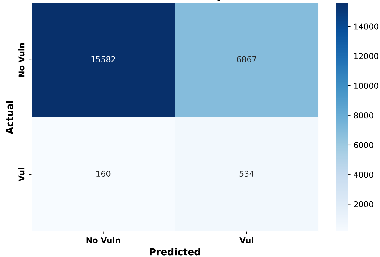
Confusion Matrix - DeepSeek-6.7B
