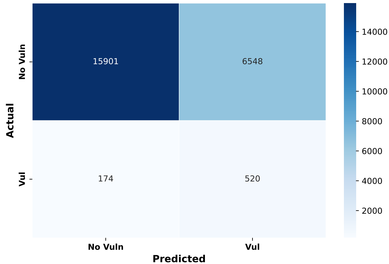
Confusion Matrix - UniXCoder Base
