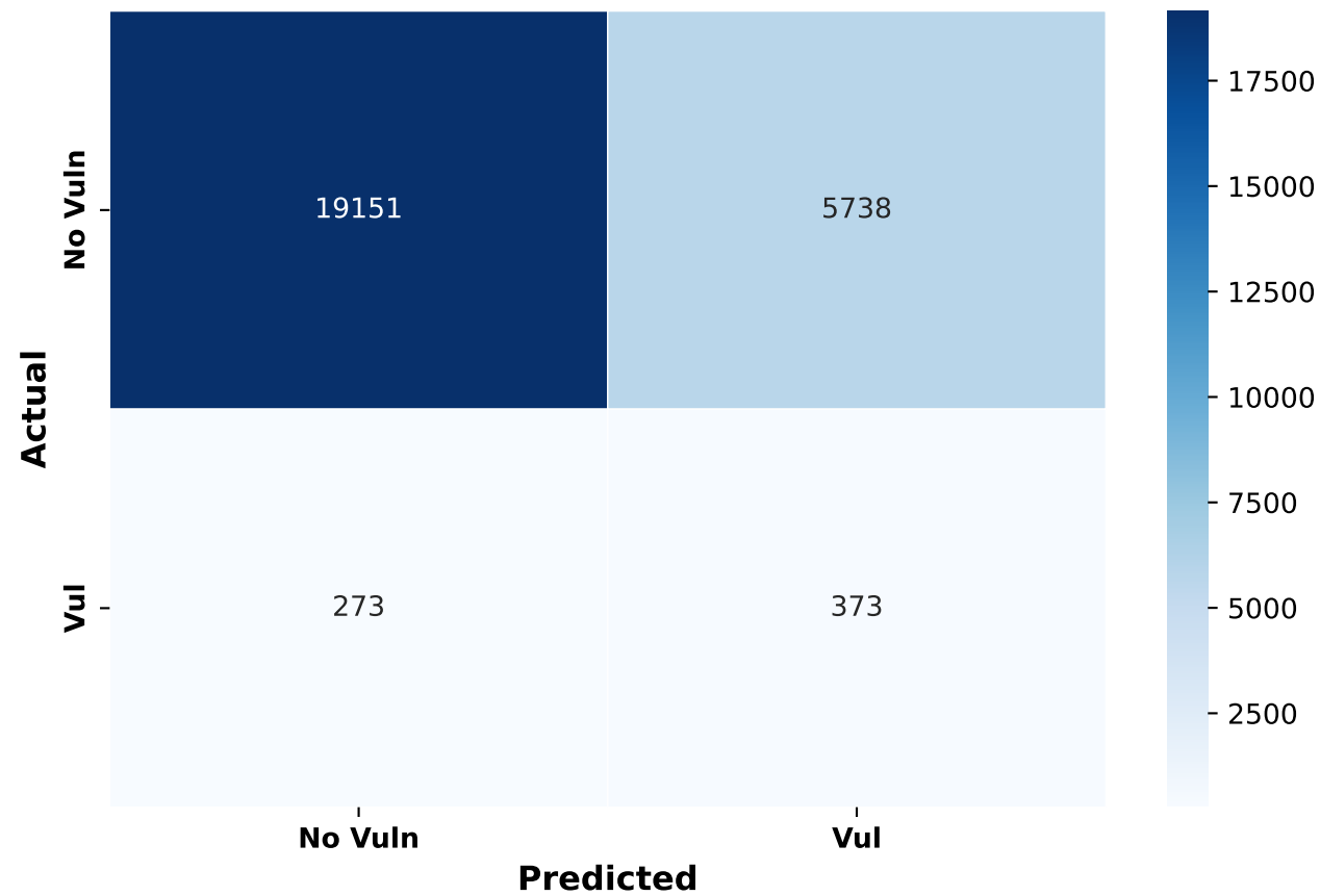
Confusion Matrix - UniXCoder Unseen Test
