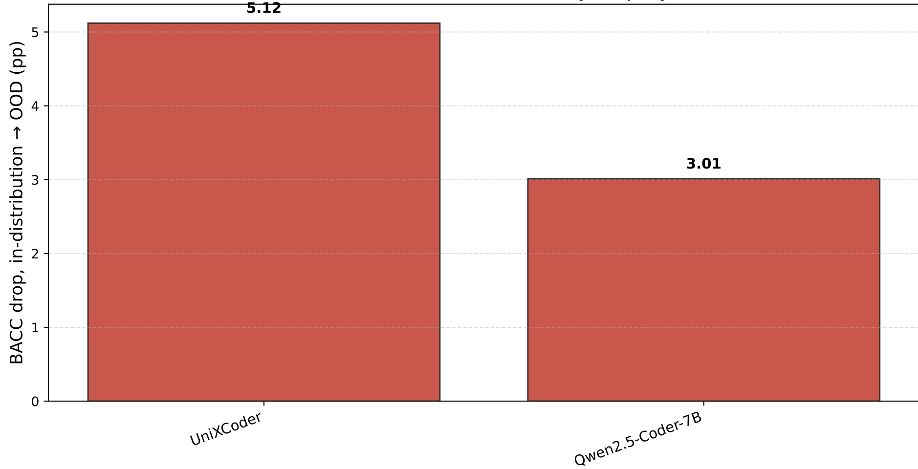
Out-of-Distribution Generalizability Gap by Model
