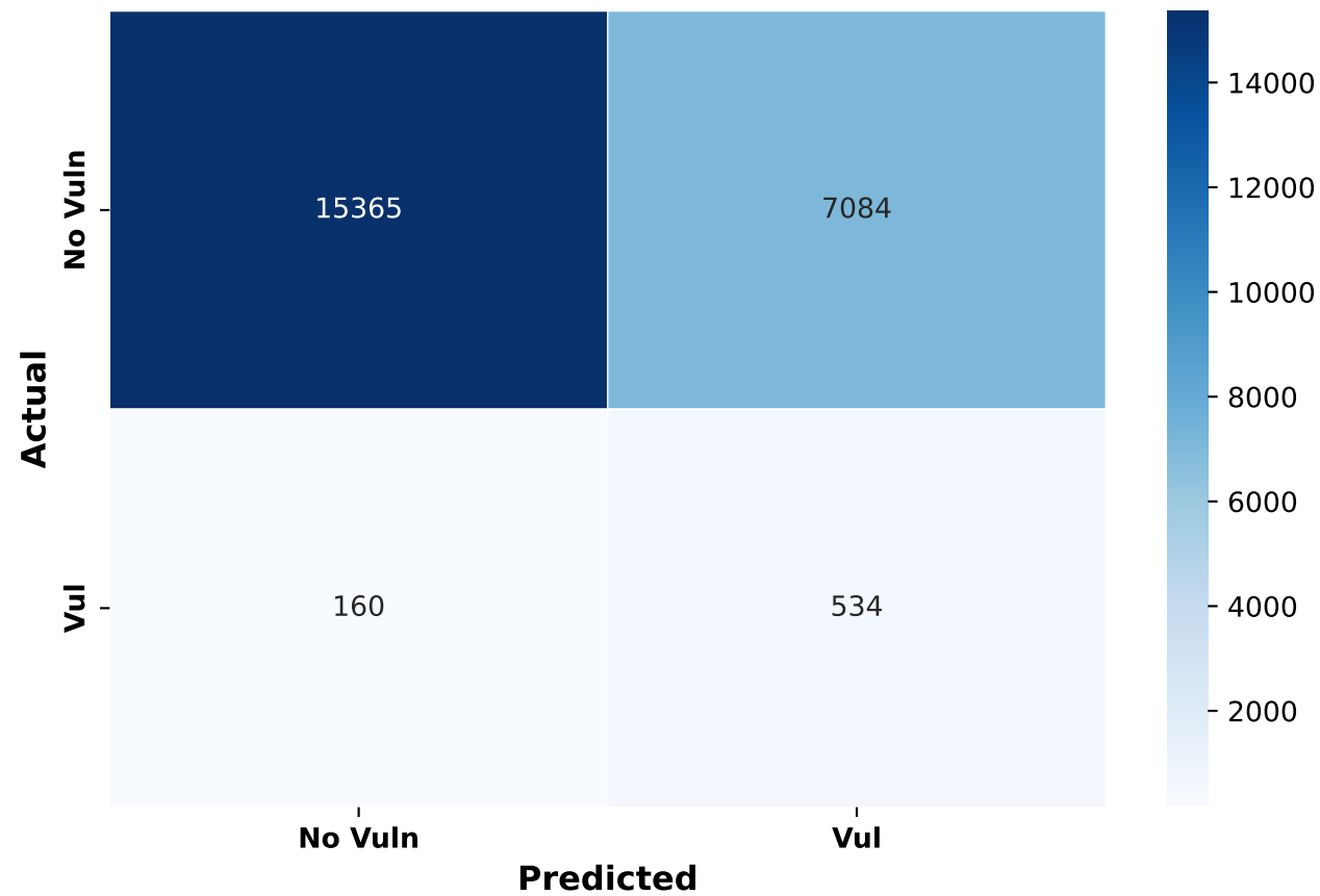
Confusion Matrix - Phi-3.5-mini
