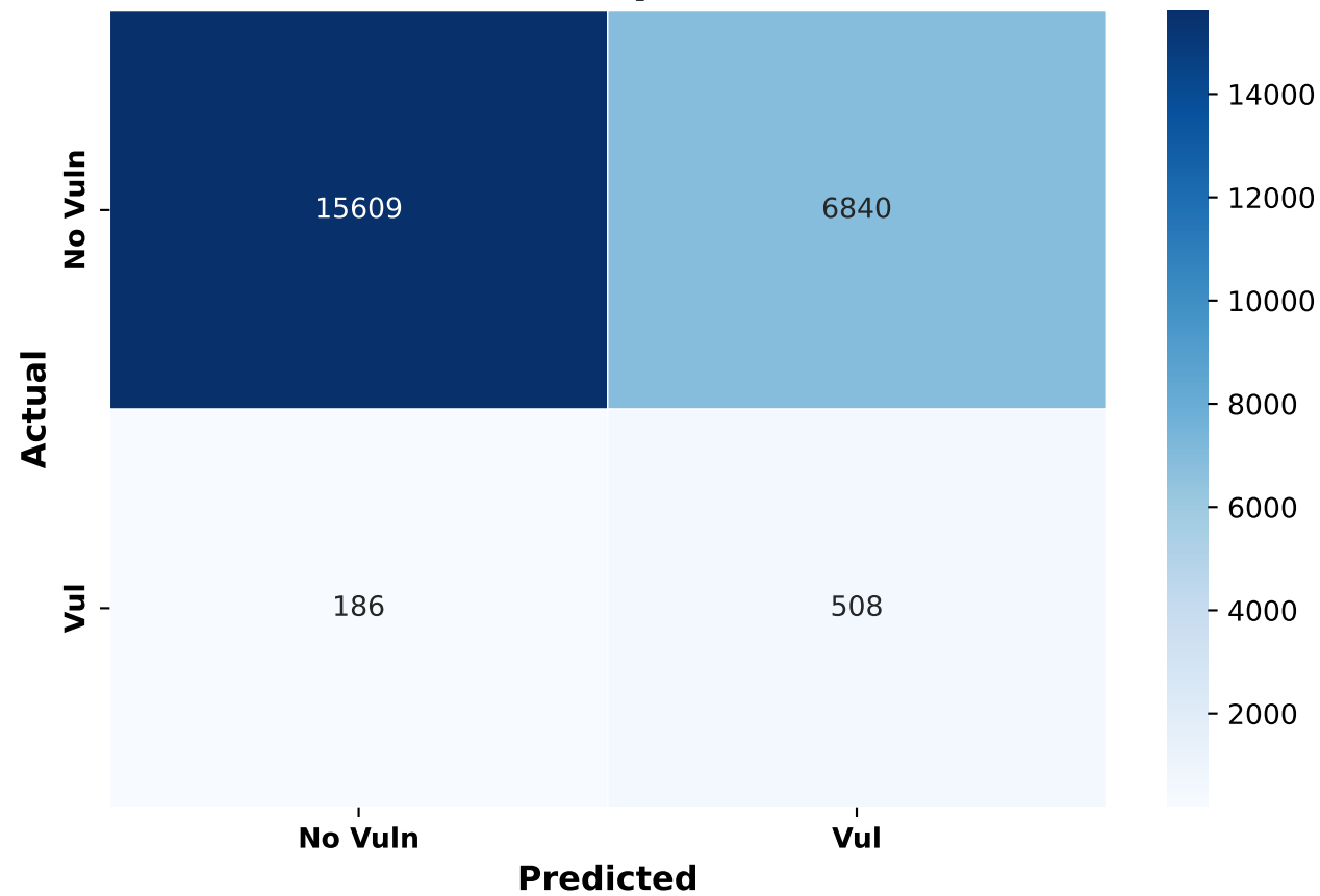
Confusion Matrix - Qwen2.5-Coder-7B
