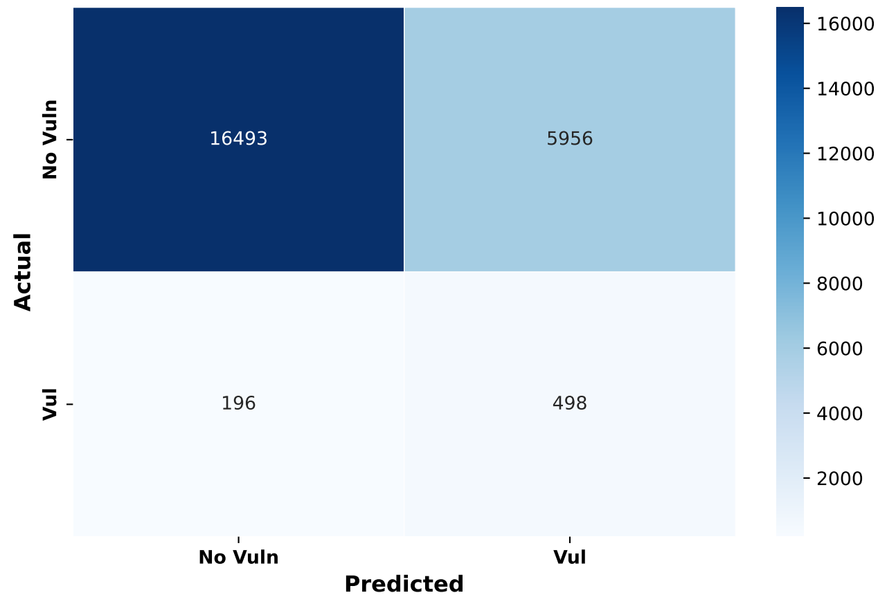
Confusion Matrix - UniXCoder No Norm
